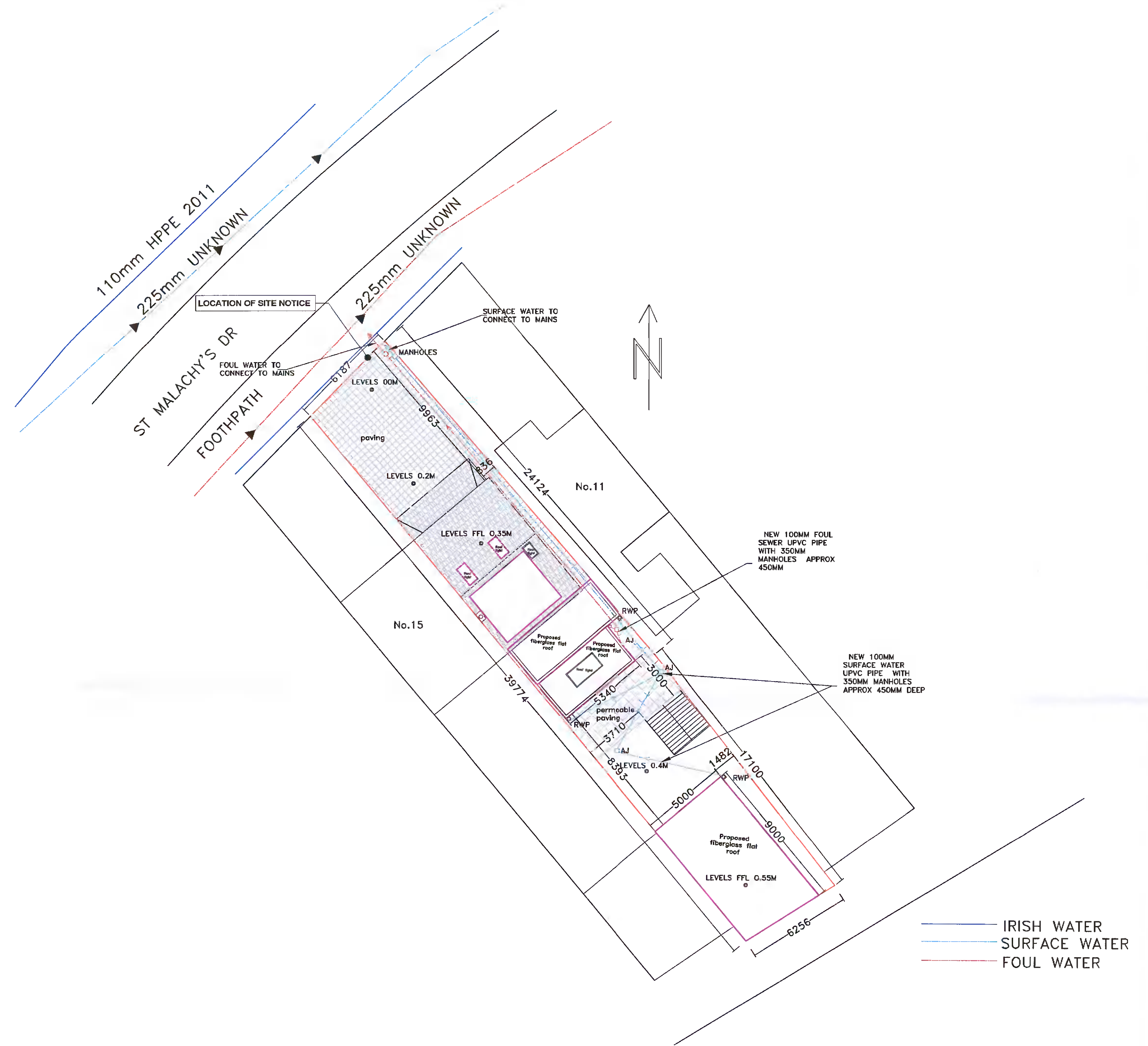
SITE LAYOUT PLAN (PROPOSED) SCALE 1:150
