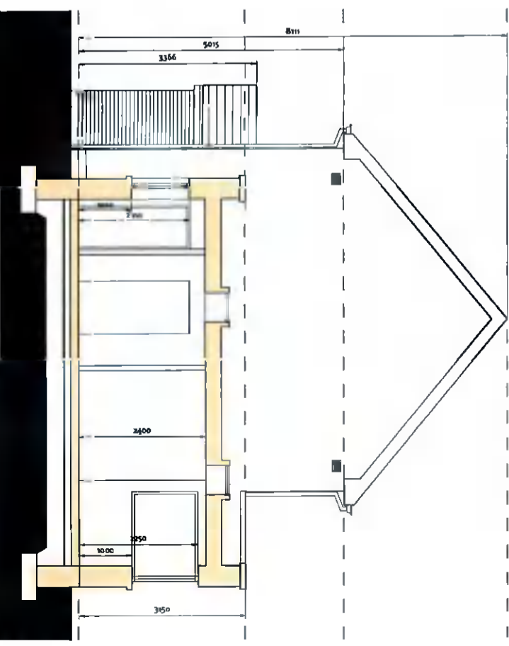
SECTION B-B PROPOSED
