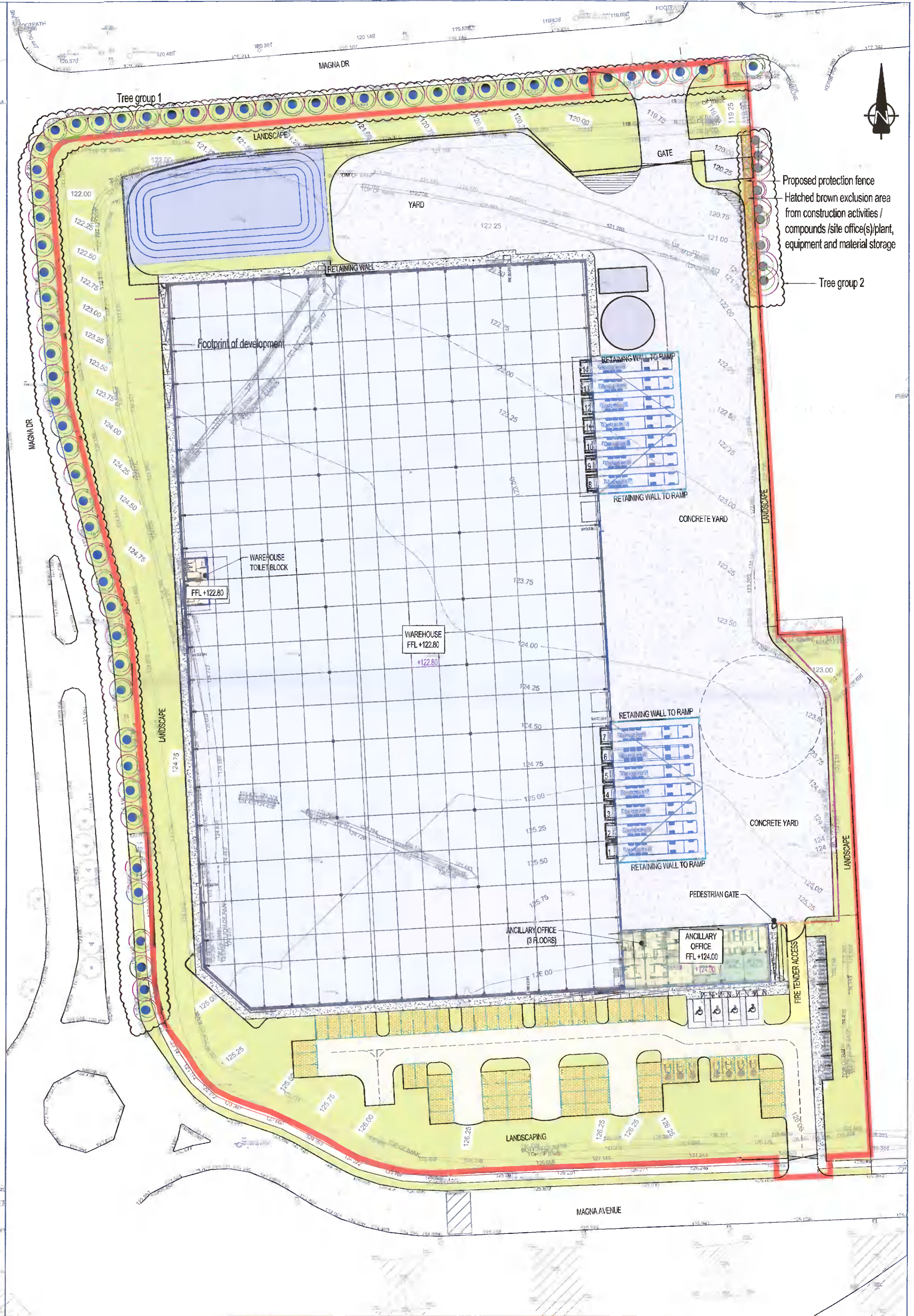
Tree Protection Plan Scale: 1:500
