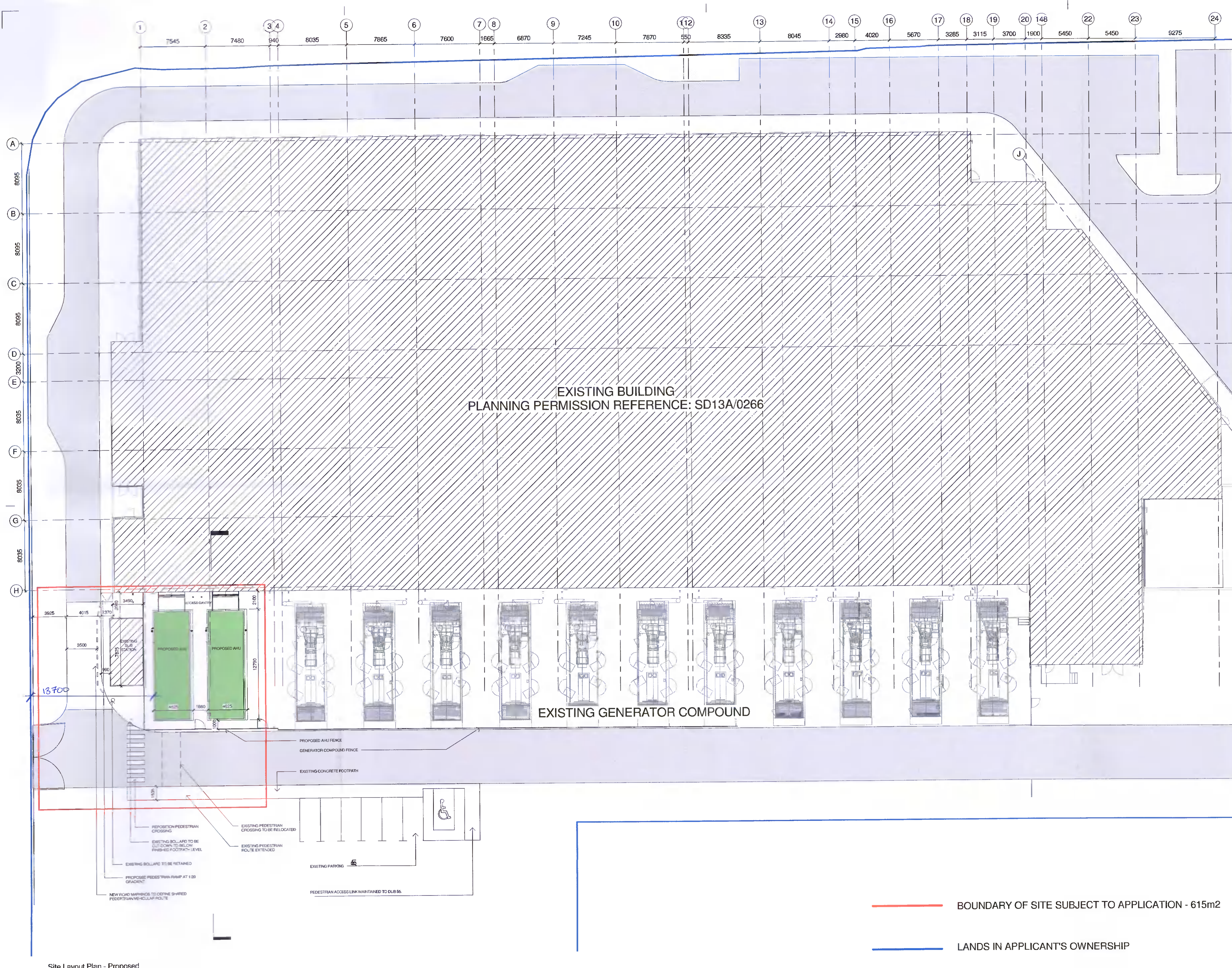
Site Layout Plan - Proposed 1 : 200
