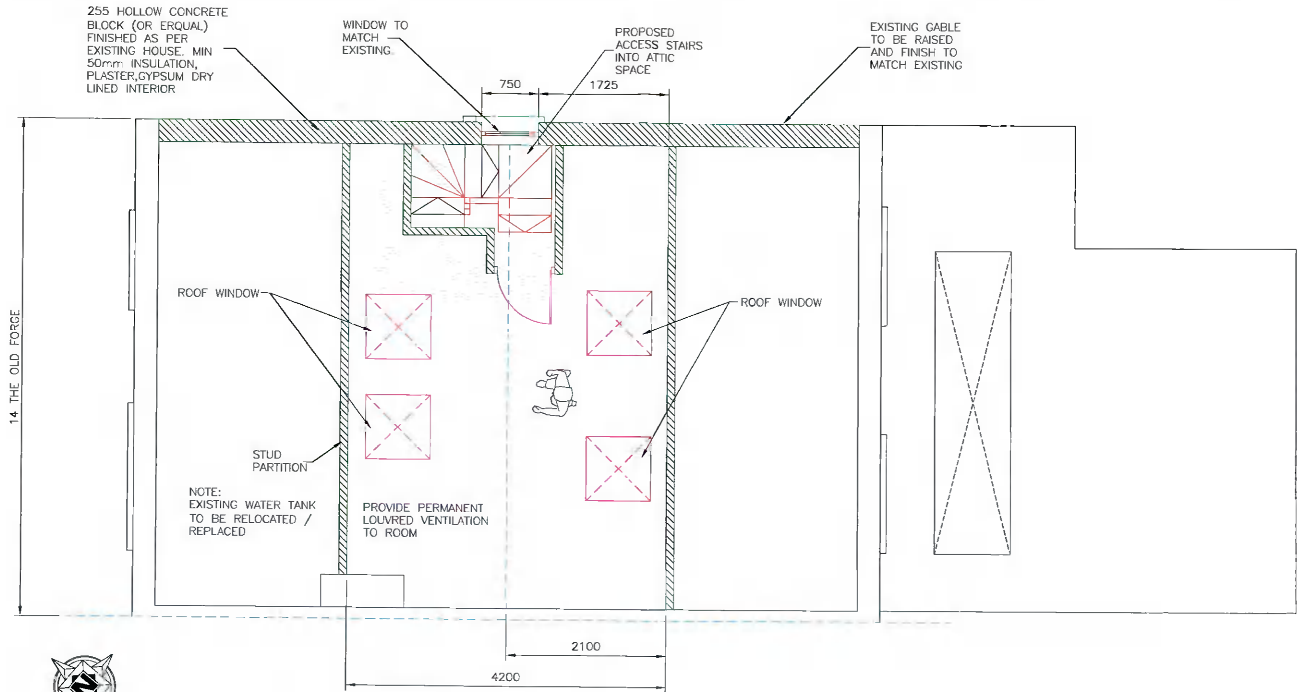
PROPOSED ATTIC FLOOR PLAN VIEW
