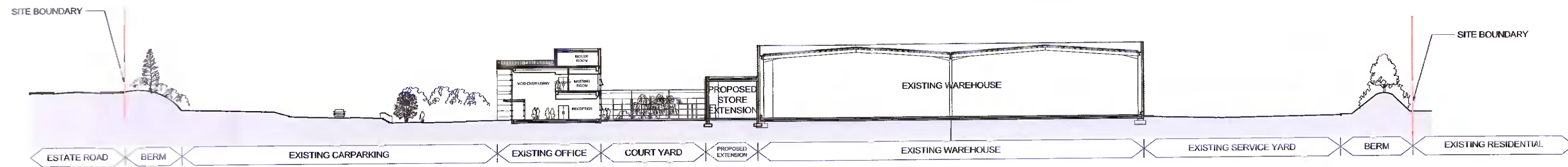
PROPOSED SITE SECTION A-A SCALE 1:500
