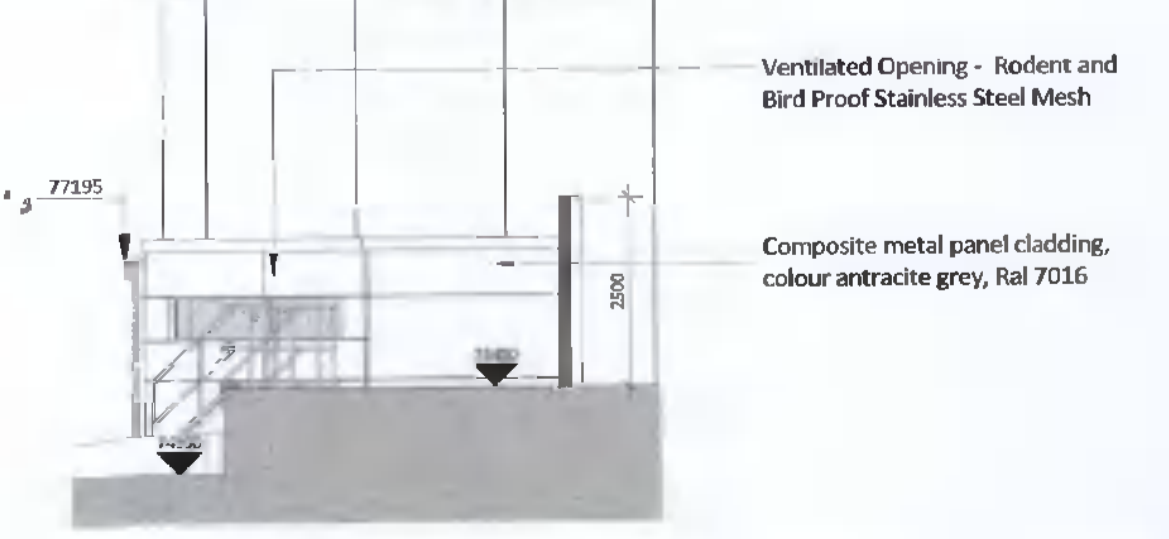
5 Waste Compound - East Elevation 1 : 100
