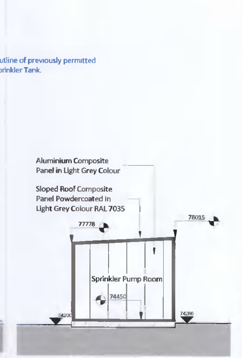
12 Sprinkler Plant - Section 1 : 100
