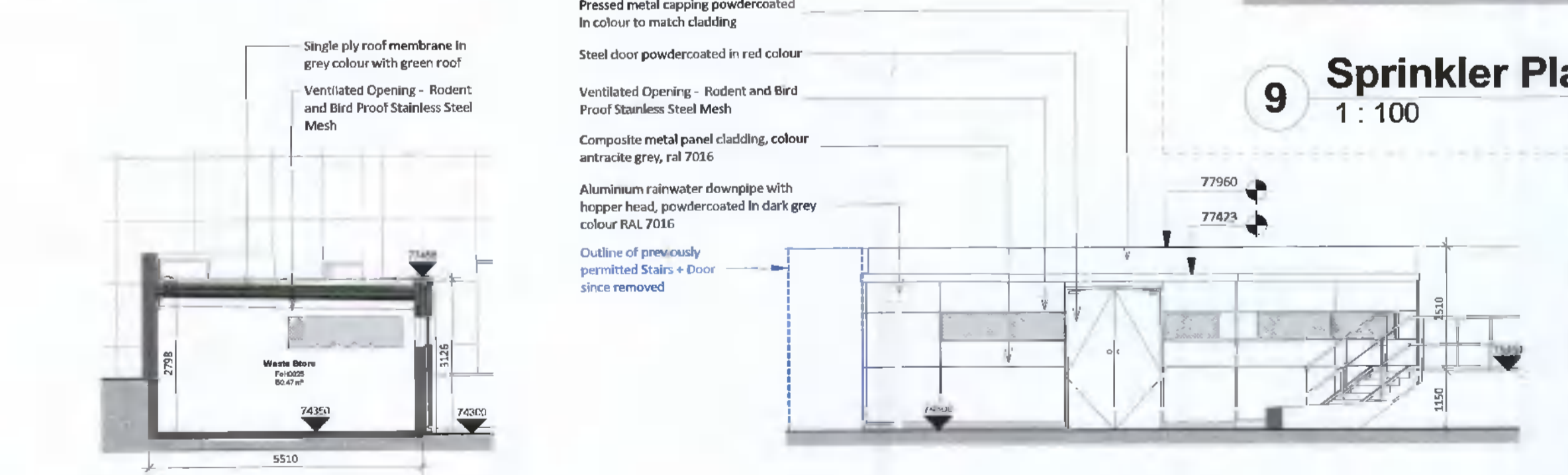
3 Waste Compound Section 1 : 100
