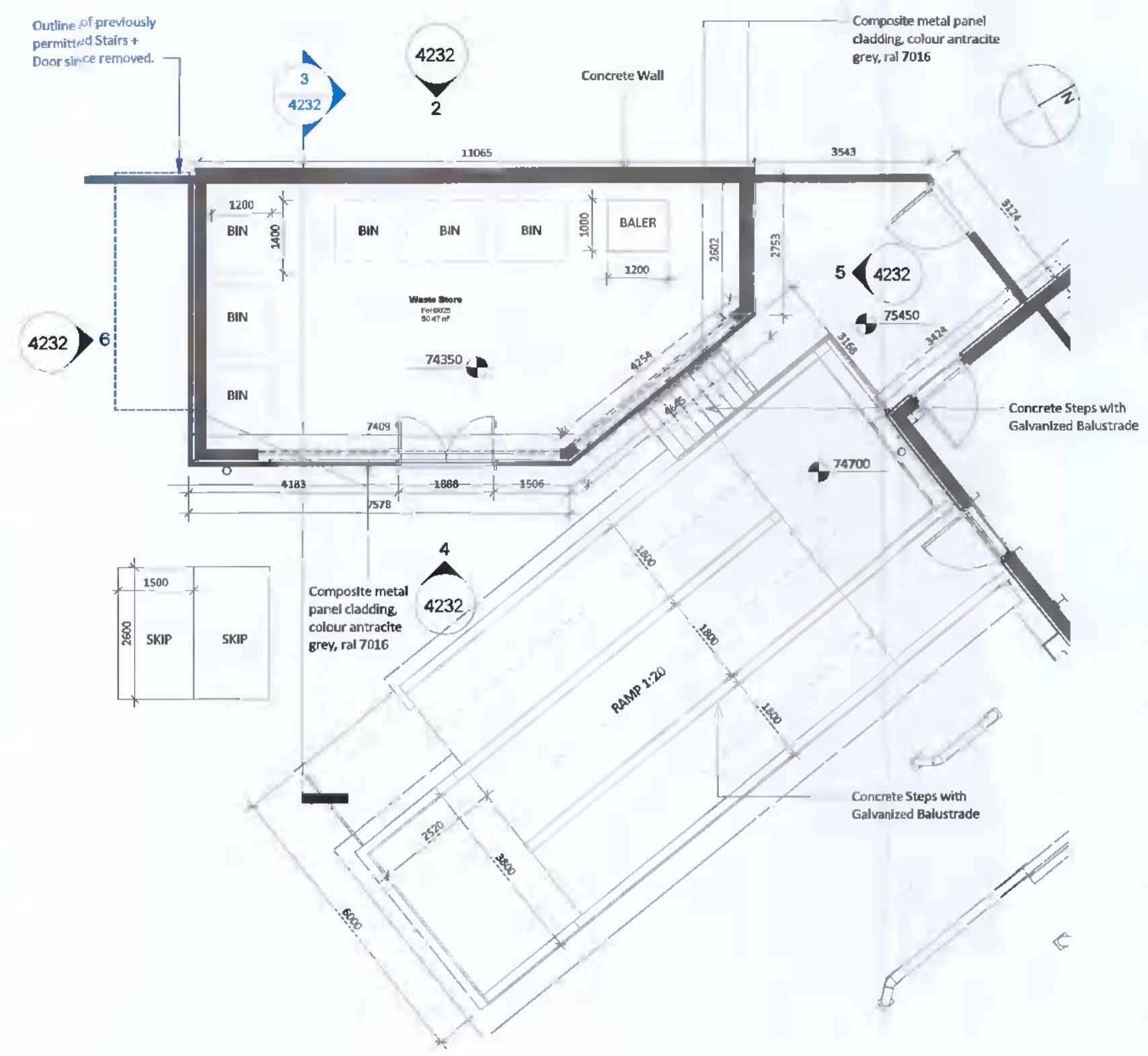
1 Waste Compound Plan 1 : 100
