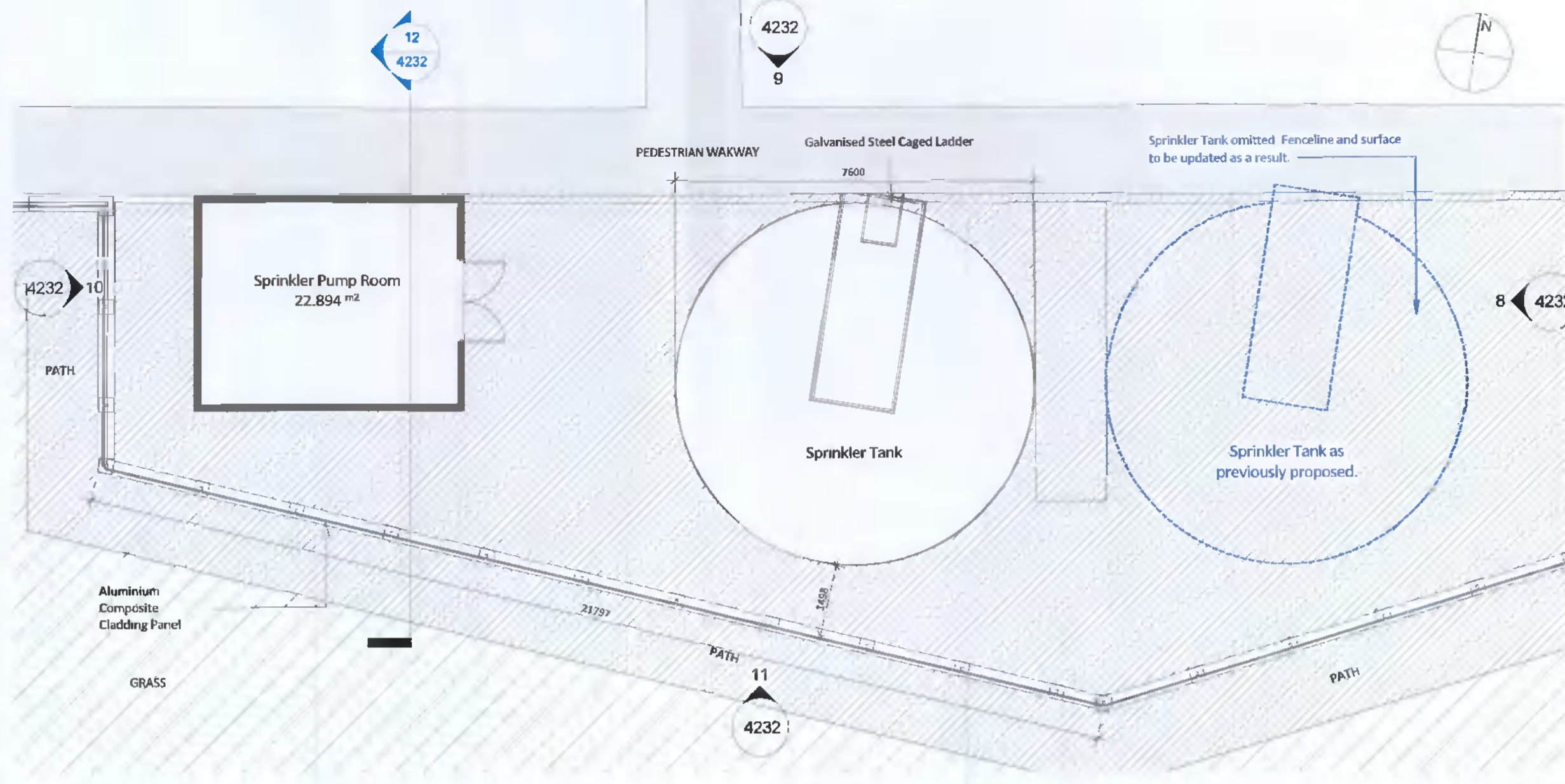
7 Sprinkler Pump Room Plan 1 : 100
