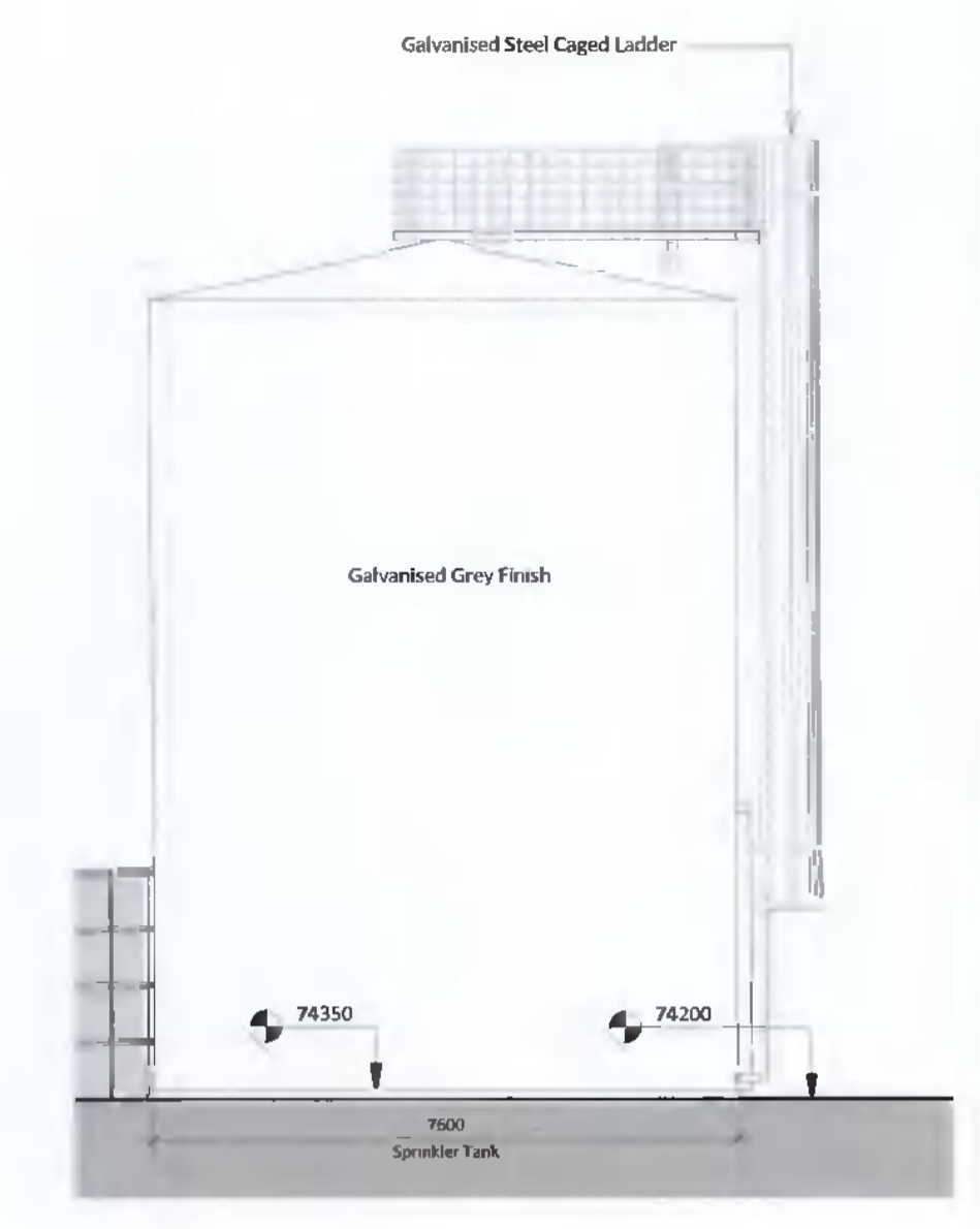
8 Sprinkler Plant - East Elevation 1 : 100
