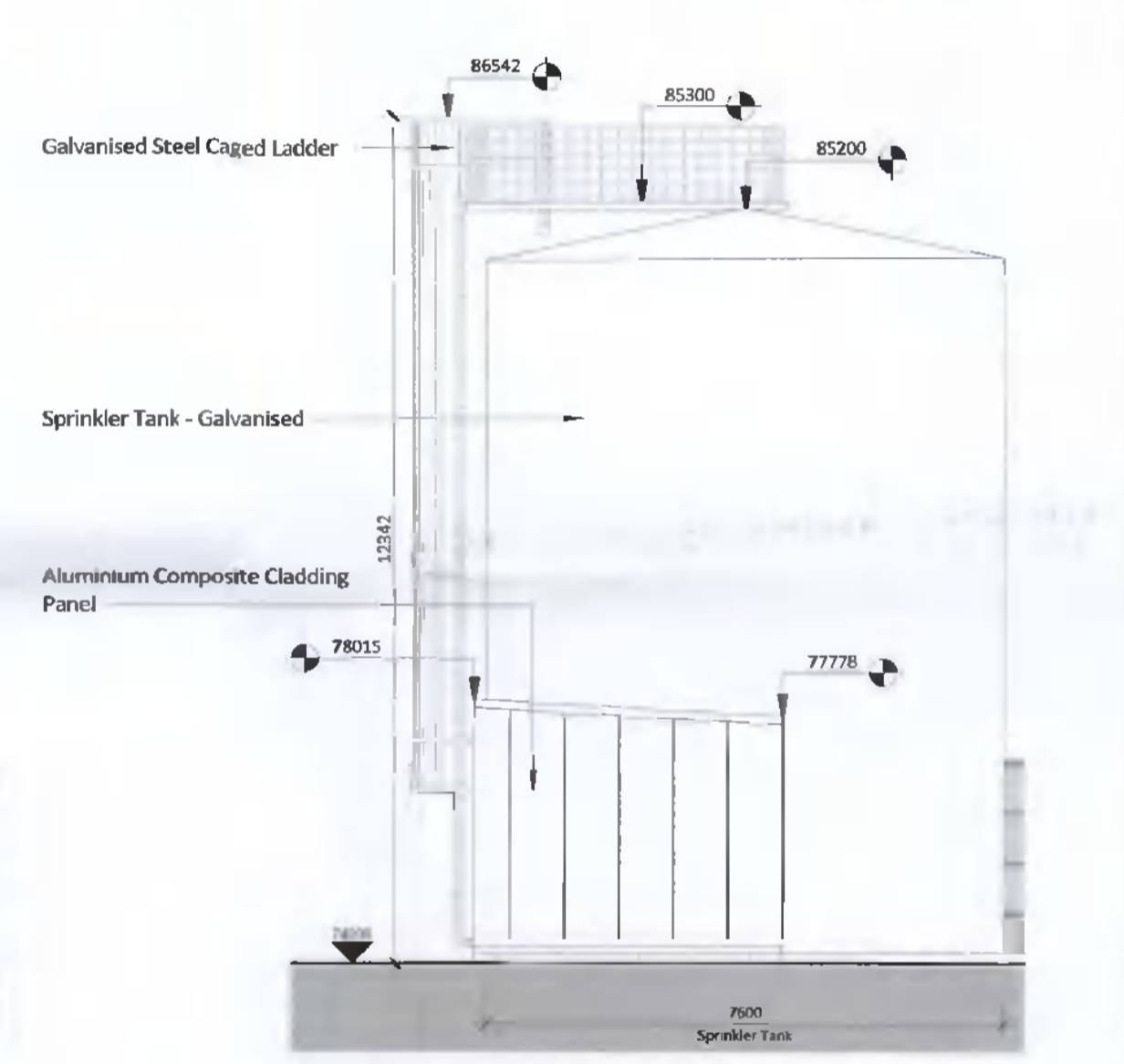
10 Sprinkler Plant - West Elevation 1 : 100
