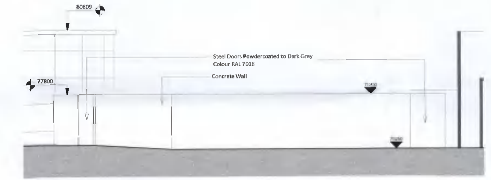
2 Waste Compound - North Elevation 1 : 100
