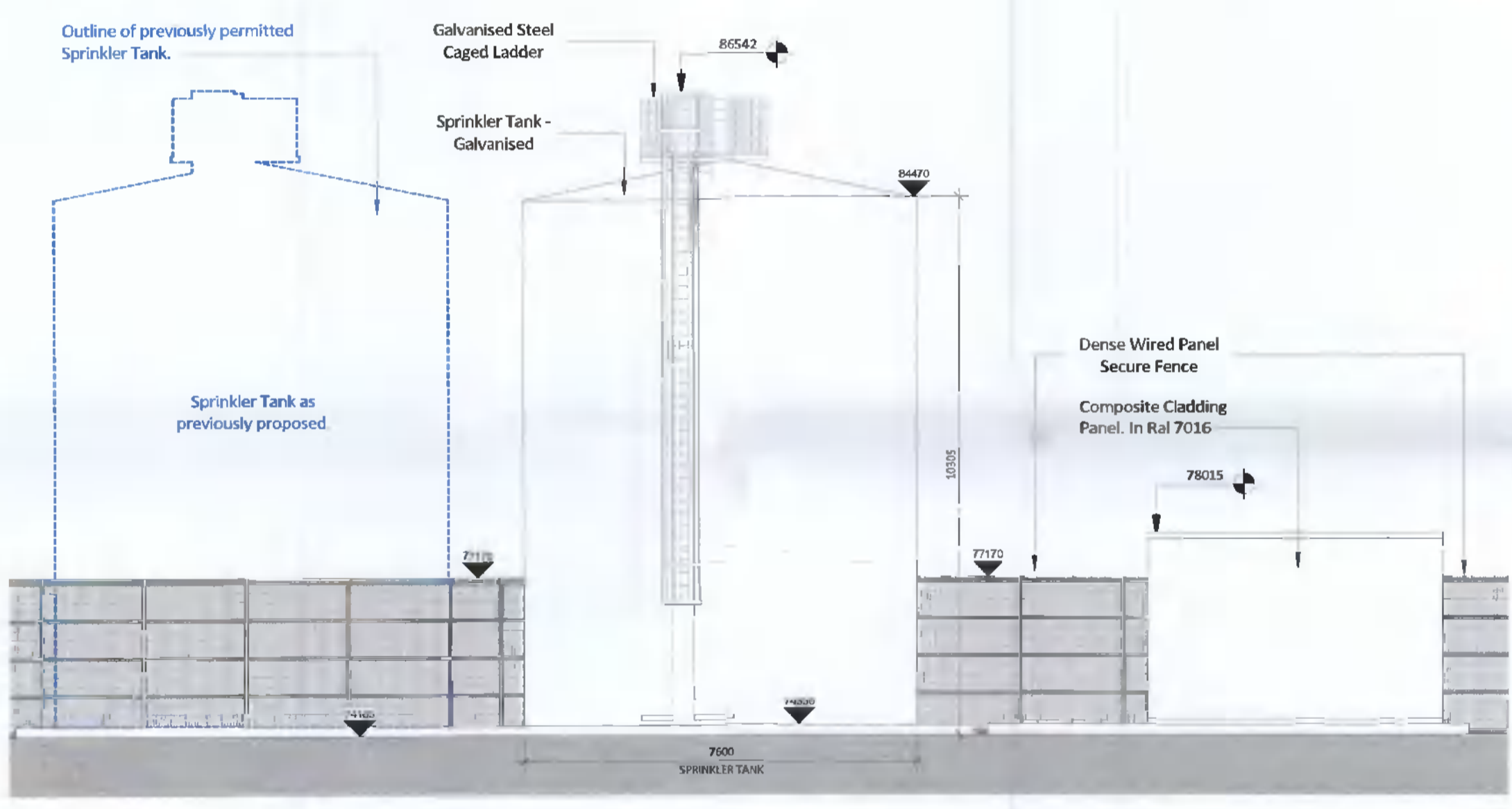
9 Sprinkler Plant - North Elevation 1 : 100
