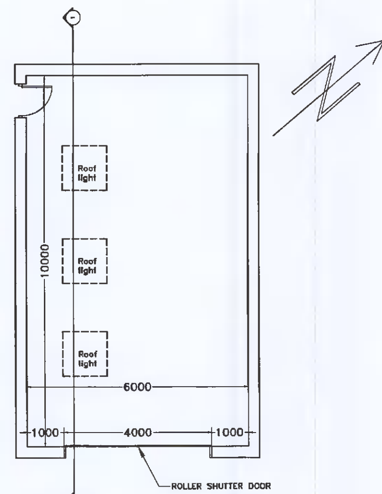
GARAGE (PROPOSED) SCALE 1:100
