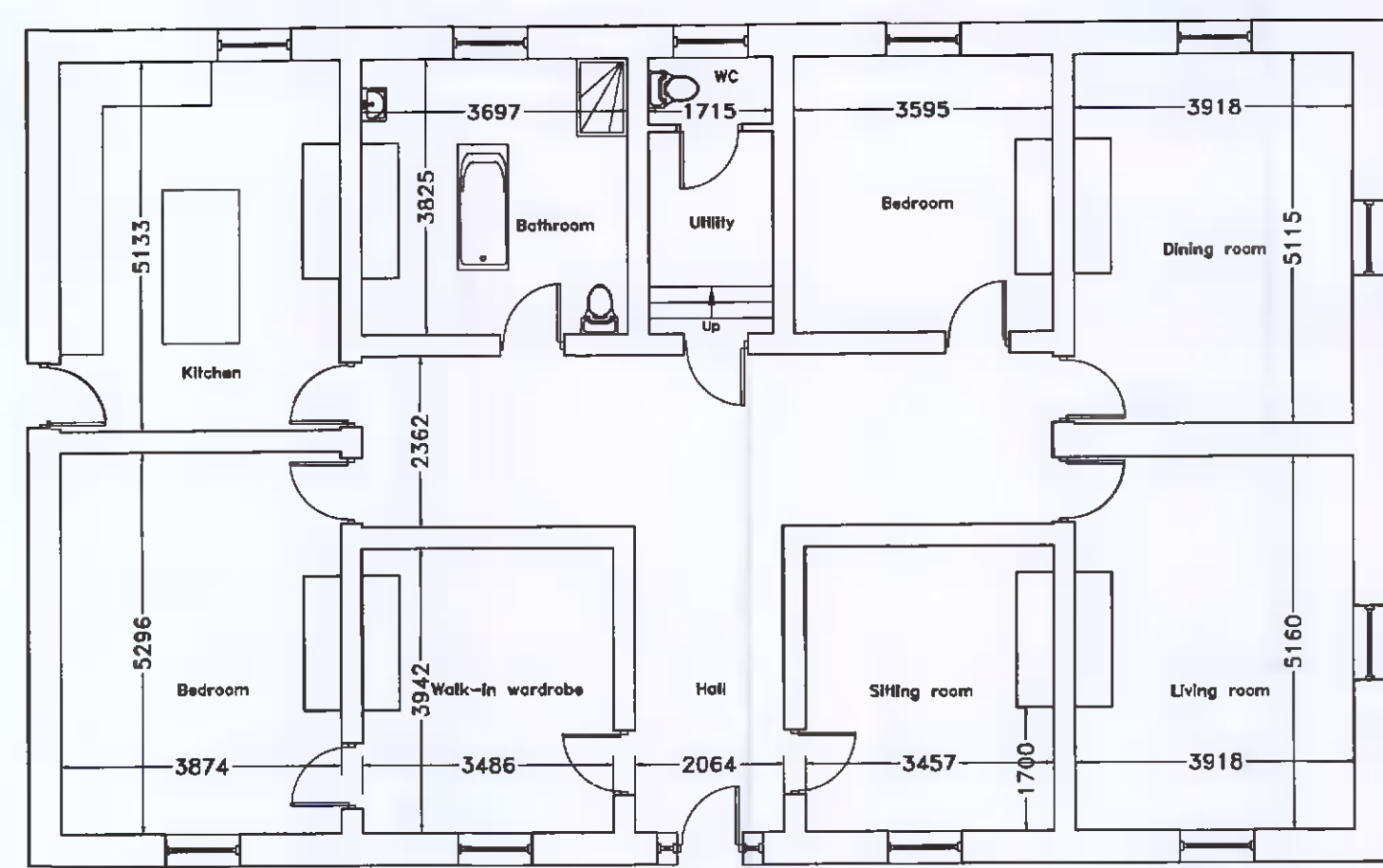
BUNGALOW (EXISTING) SCALE 1:100
