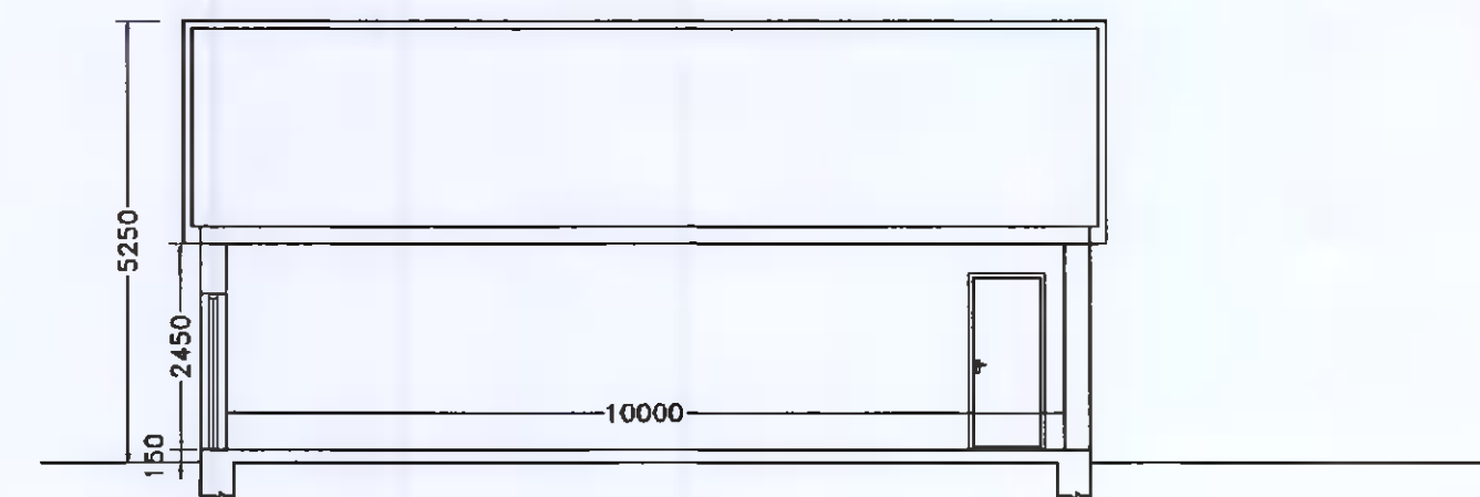
GARAGE SECTION (PROPOSED) SCALE 1:100
