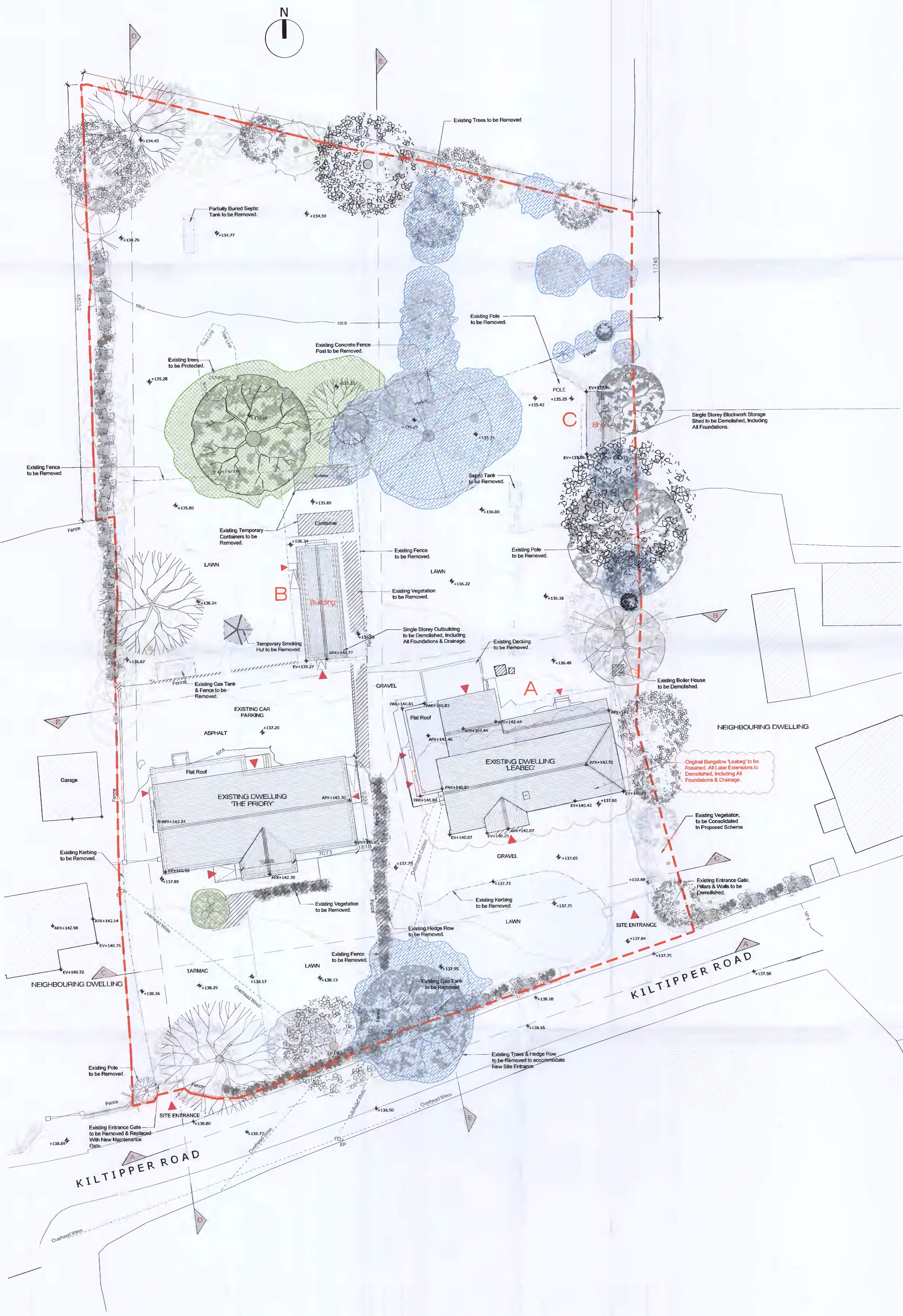
Existing Site & Demolition Plan ■ scale 1:200 @ A1
