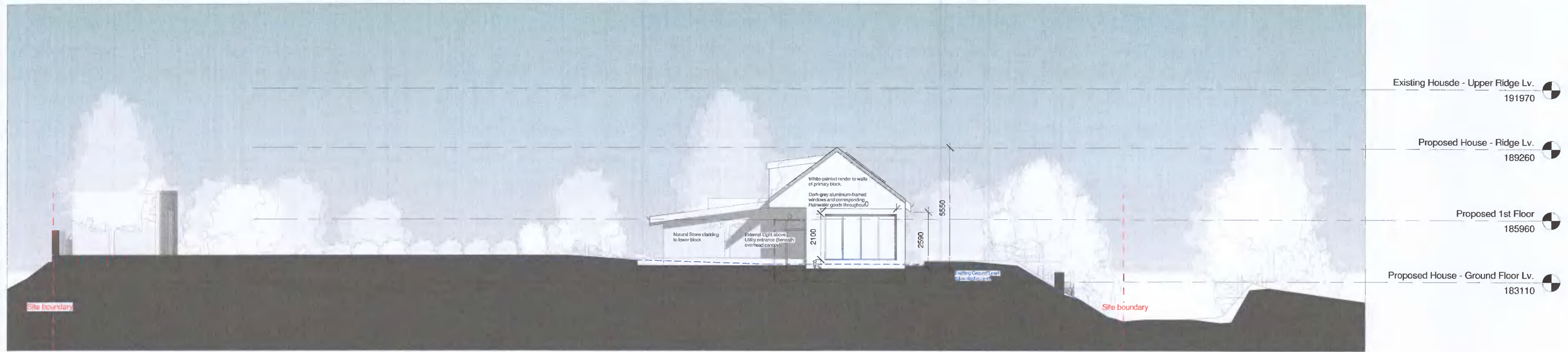
1 South-West Elevation 1 : 100
