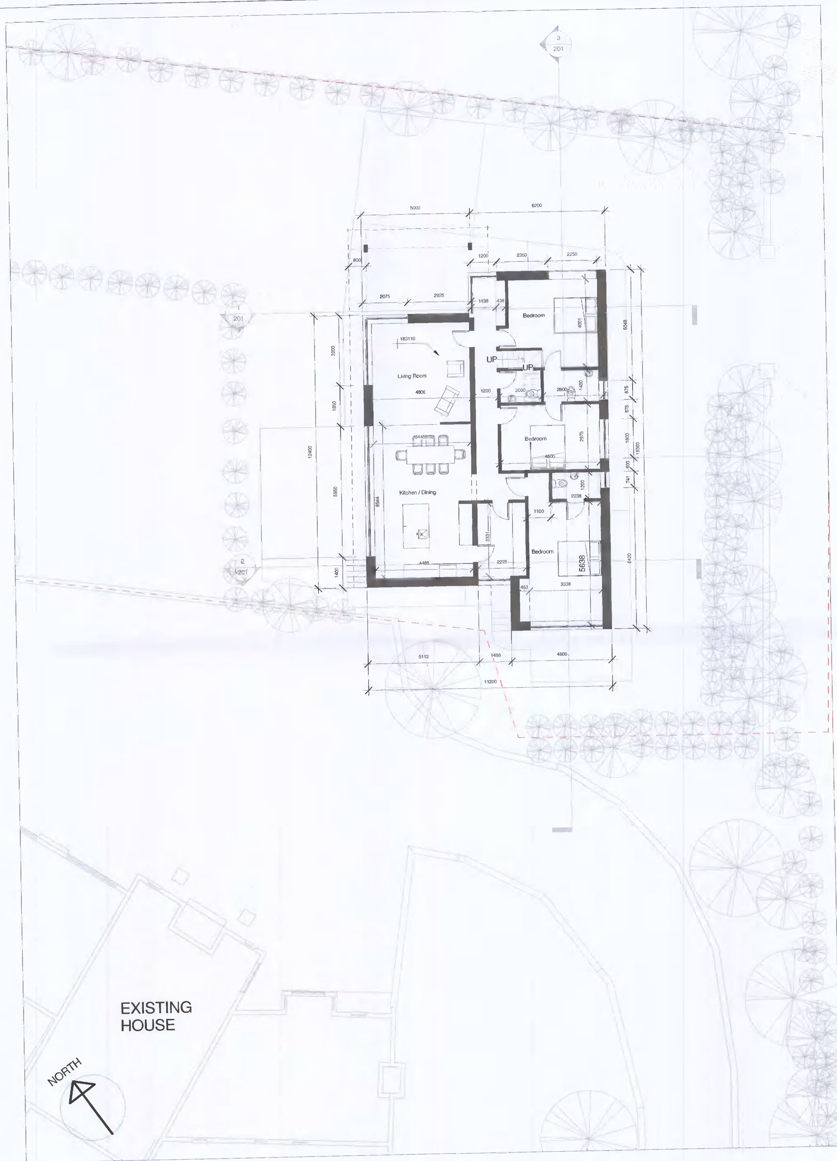
1 Proposed Ground Floor 1 : 100
