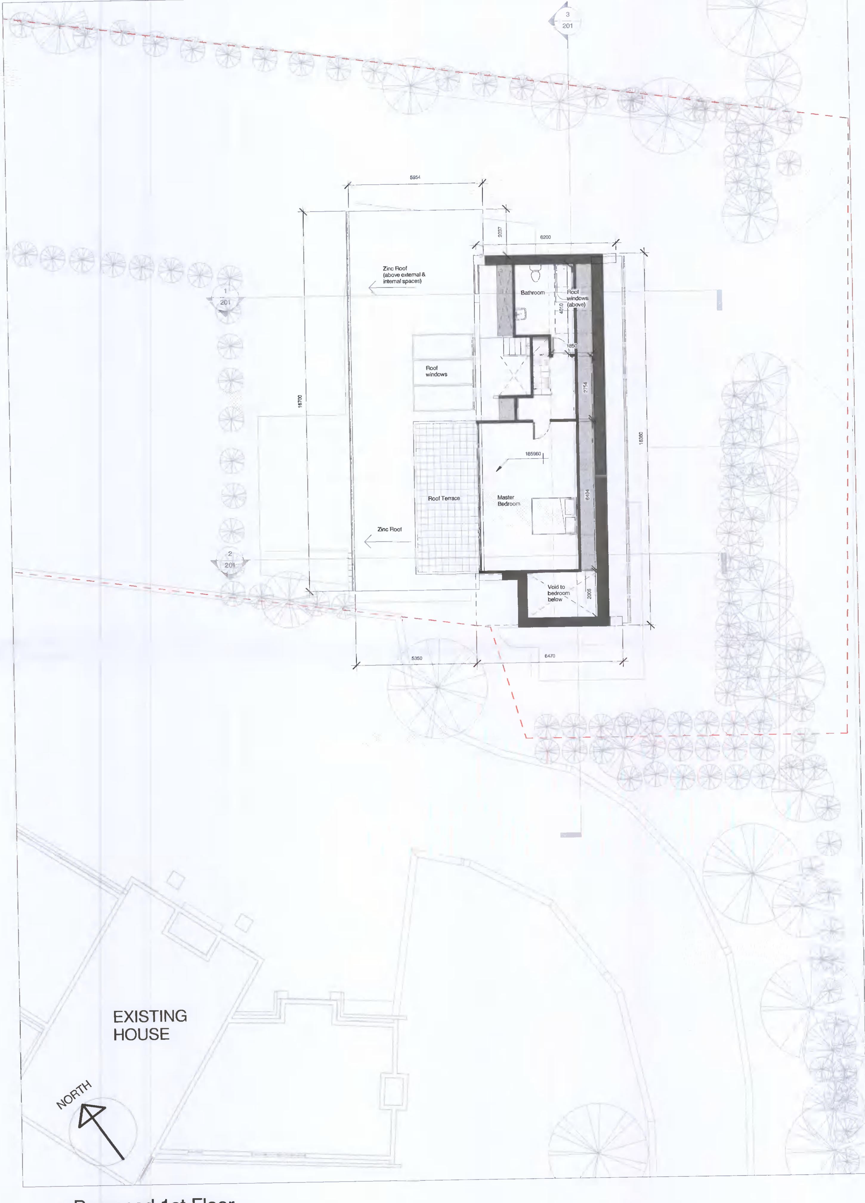
2 Proposed 1st Floor 1 : 100
