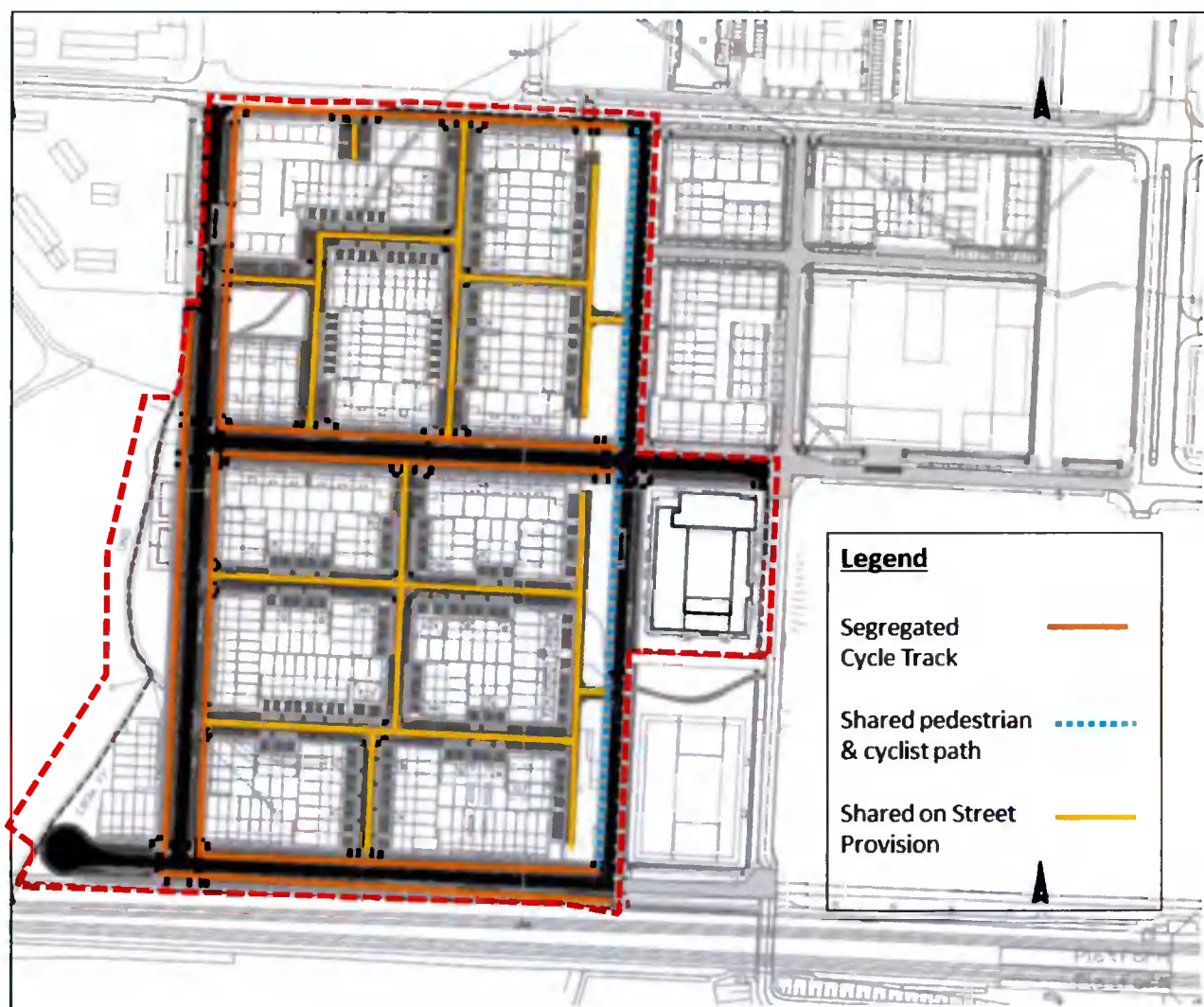
Figure 3-4 - Adamstown Boulevard Phase1 Cyclist Provision
