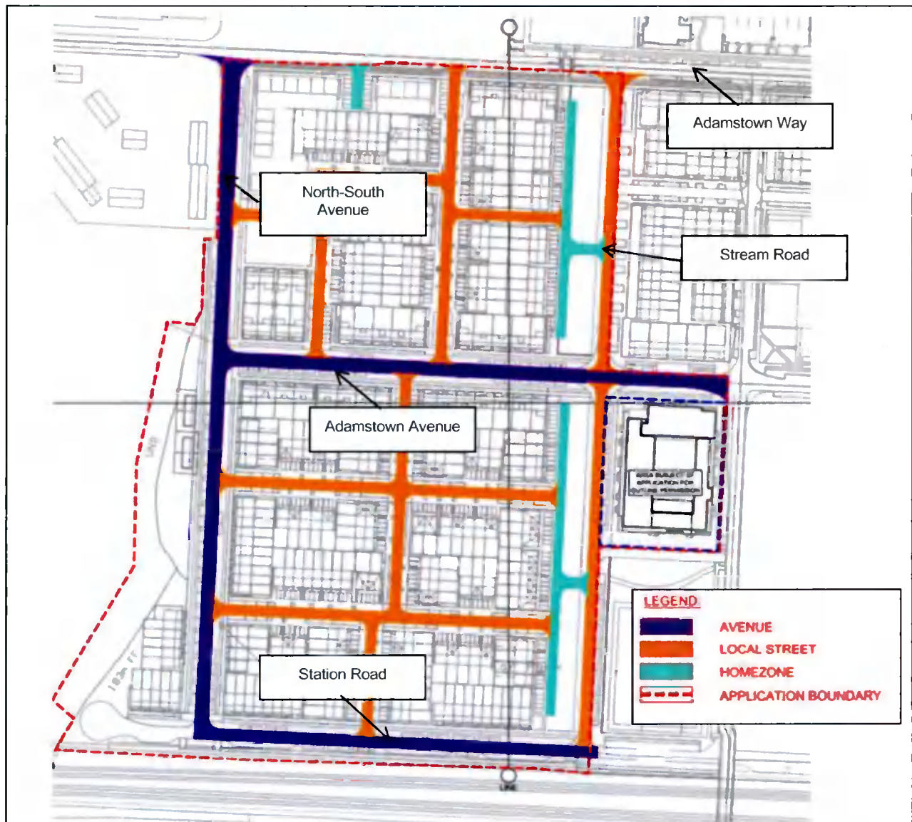
Figure 3-1 – Road Hierarchy and Street Layout
