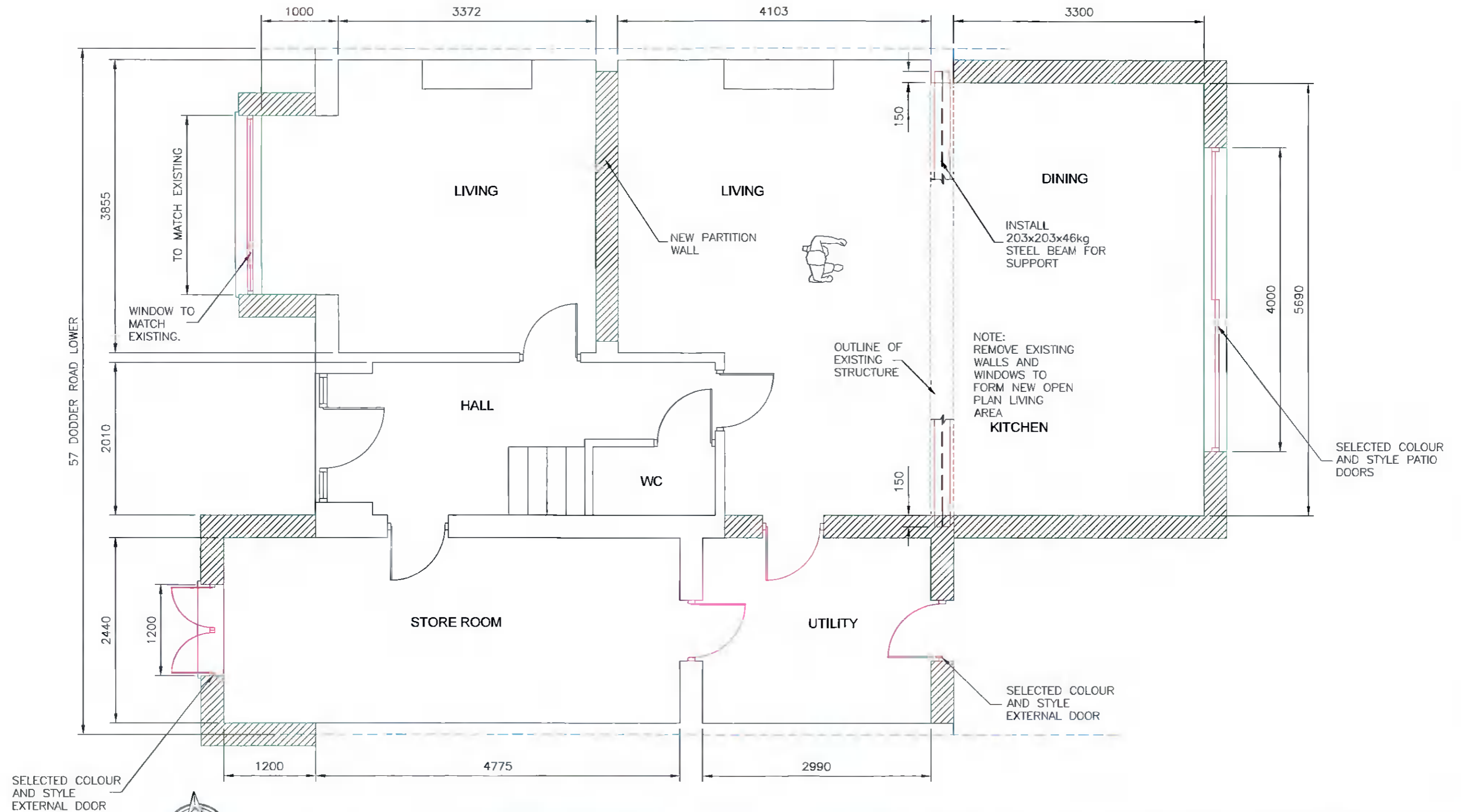
PROPOSED GROUND FLOOR PLAN VIEW
