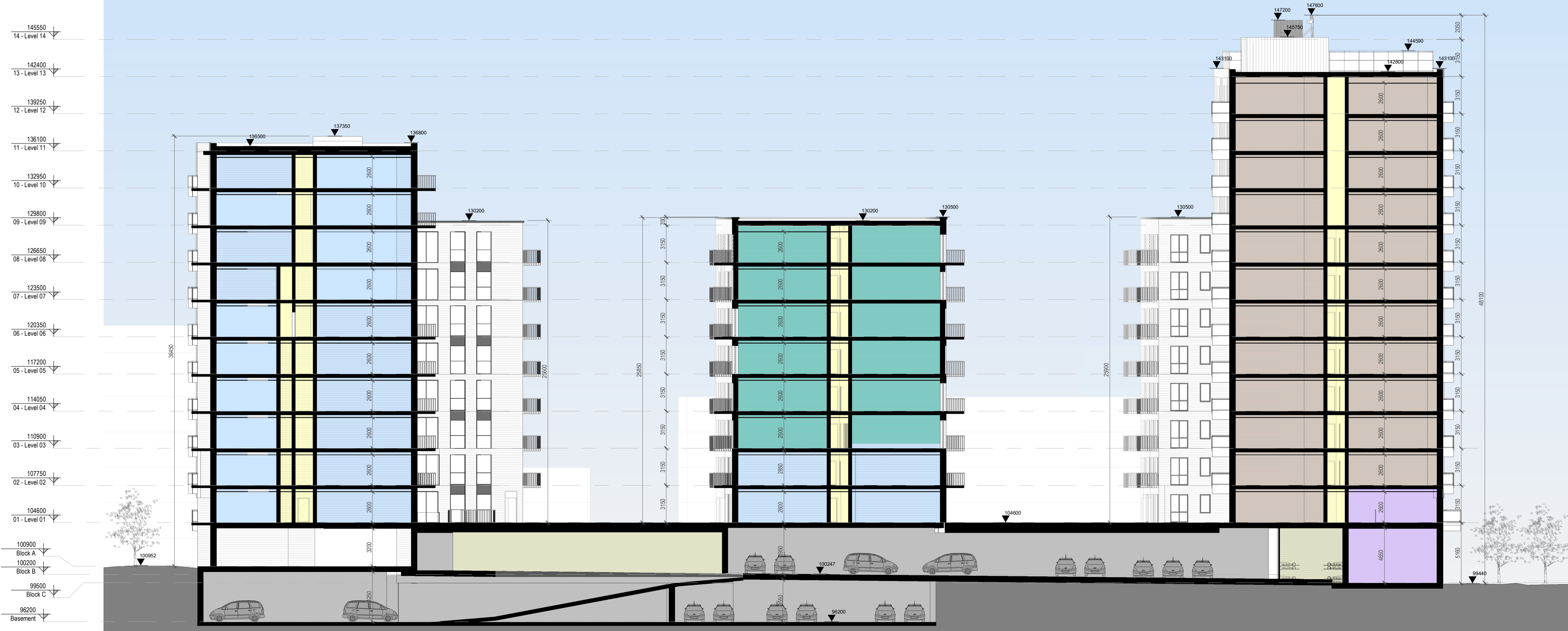
2 Section 04 1: 200
