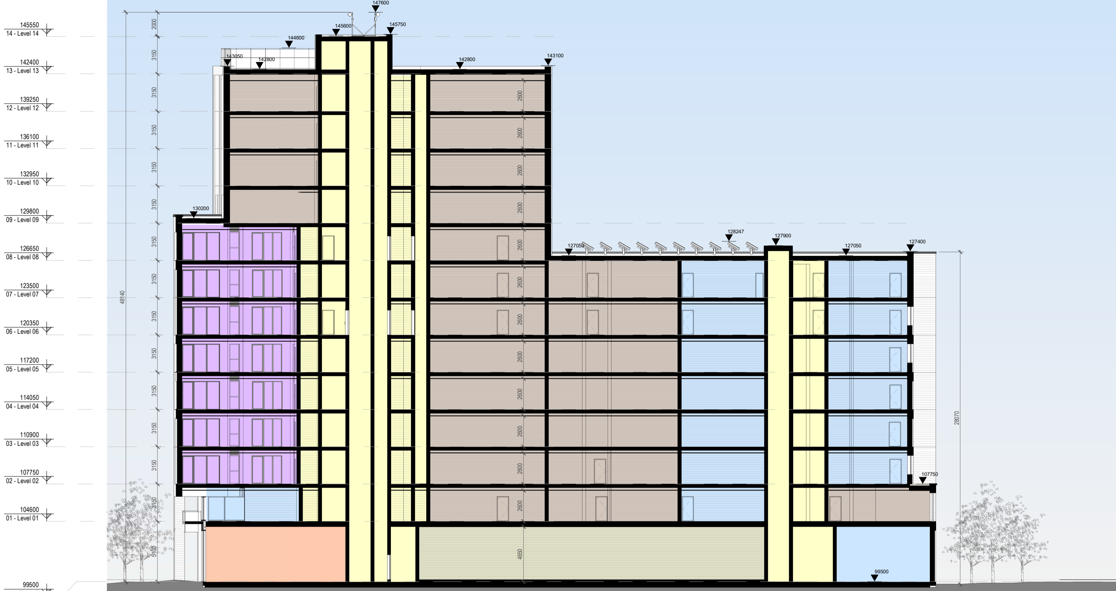
1 Section 03 1: 200
