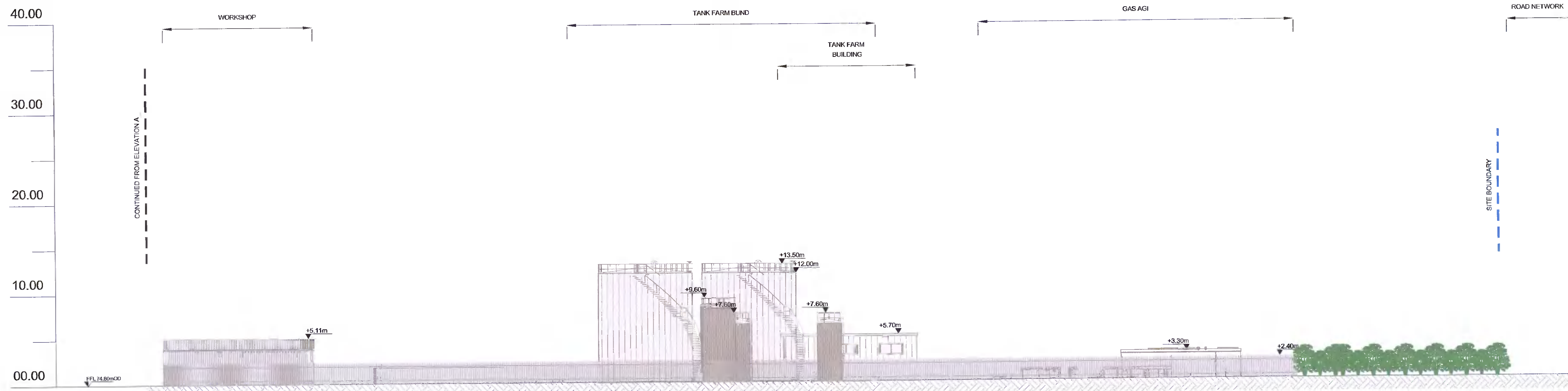
CONTIGUOUS ELEVATION B - Scale 1:250
