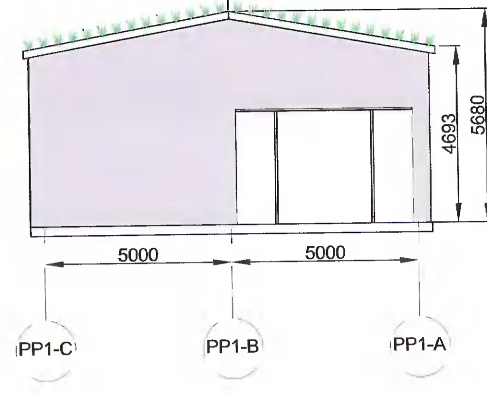
East Facing Elevation S1
