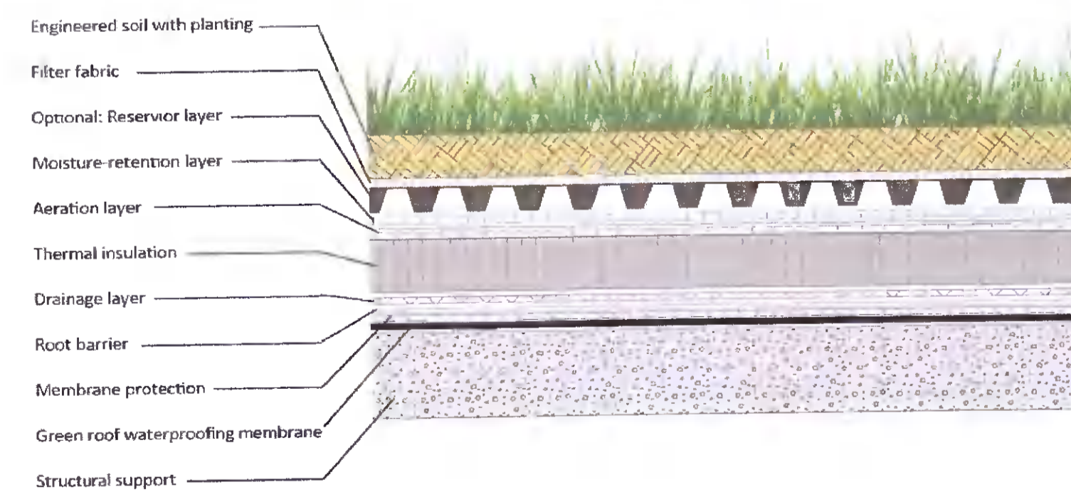
Typical Green Roof Design (TBC at Detailed design stage)
