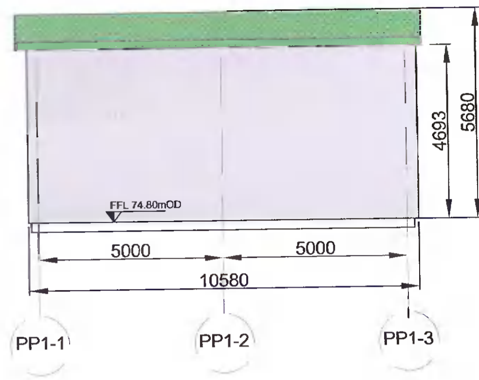
North Facing Elevation S2
