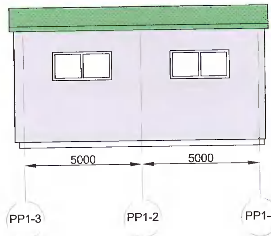
South Facing Elevation S4
