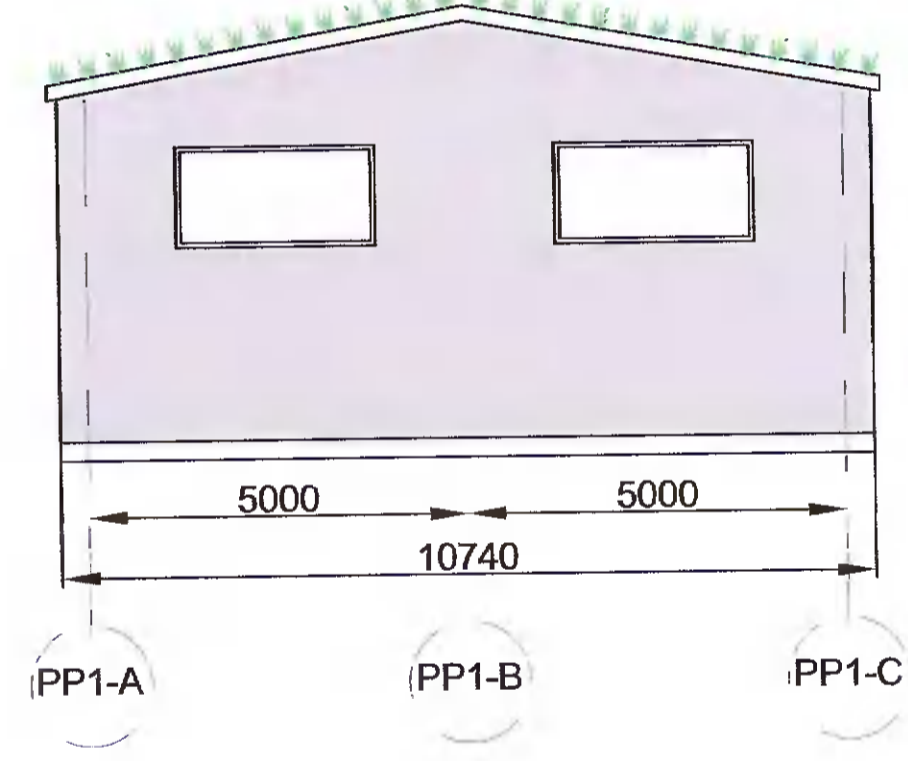
West Facing Elevation S3
