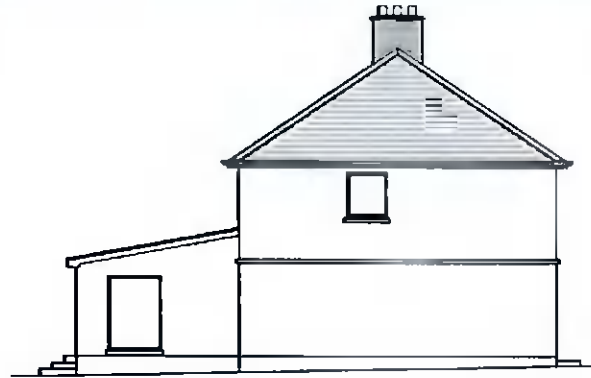
SURVEY SIDE ELEVATION Scale 1:100
