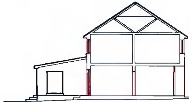
SURVEY SECTION Scale 1:100
