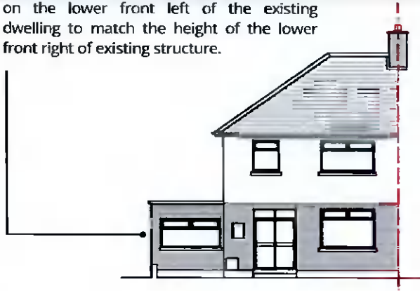
SURVEY FRONT ELEVATION Scale 1:100
