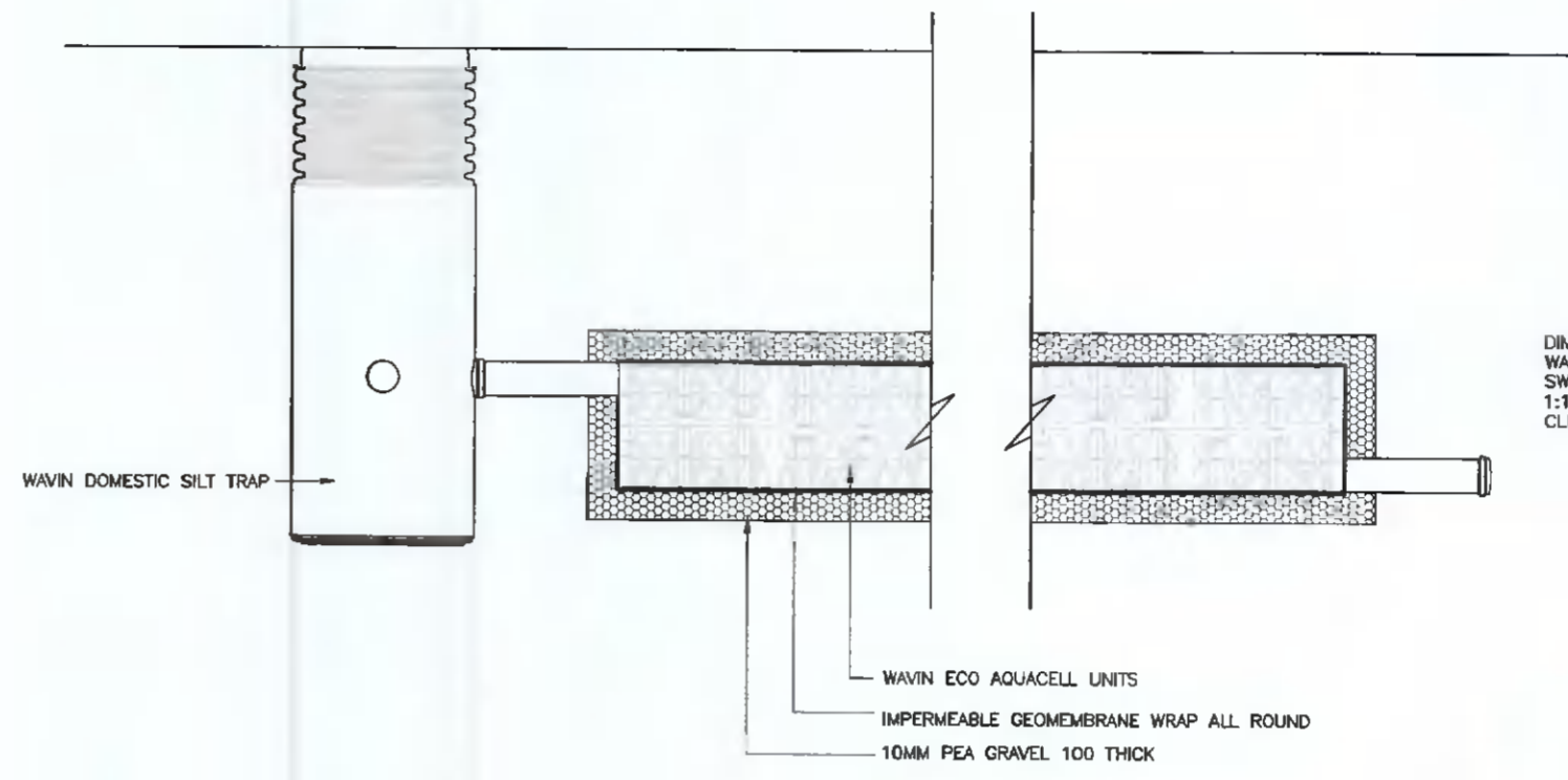
TYPICAL SECTION THRU DOMESTIC SW ATTENUATION
