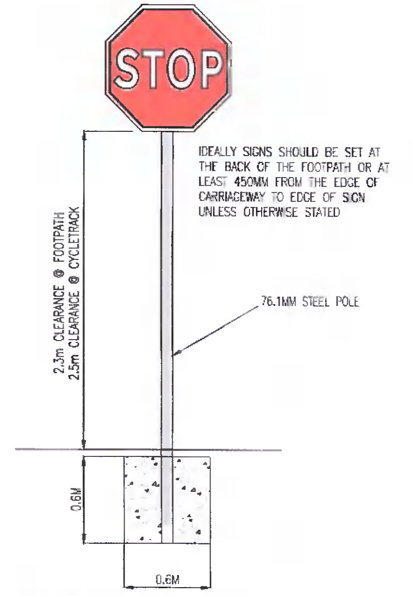
TYPICAL MOUNTING ARRANGEMENT IN FOOTPATHS INCLUDING FOUNDATION DETAILS N.T.S.
