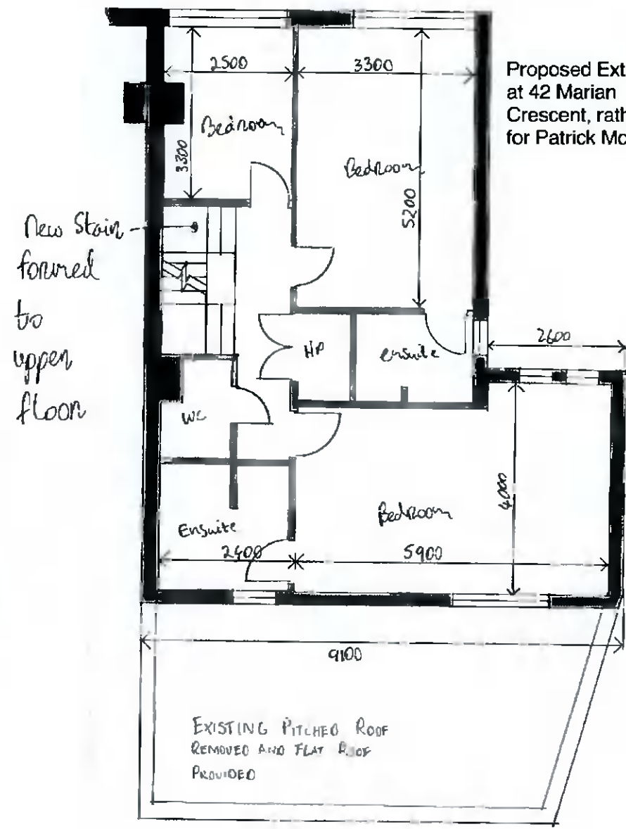
Existing/Proposed first floor Plan 1:100
