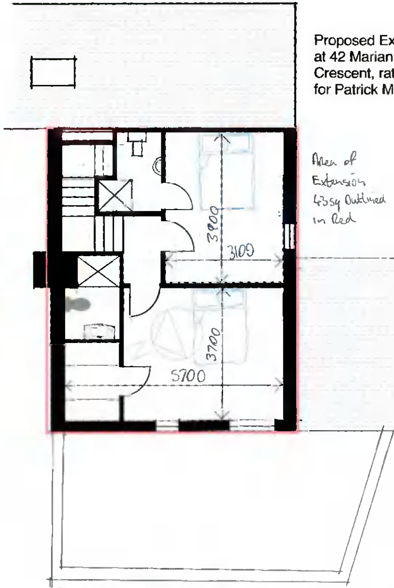
PROPOSED SECOND FLOOR PLAN 1:100
