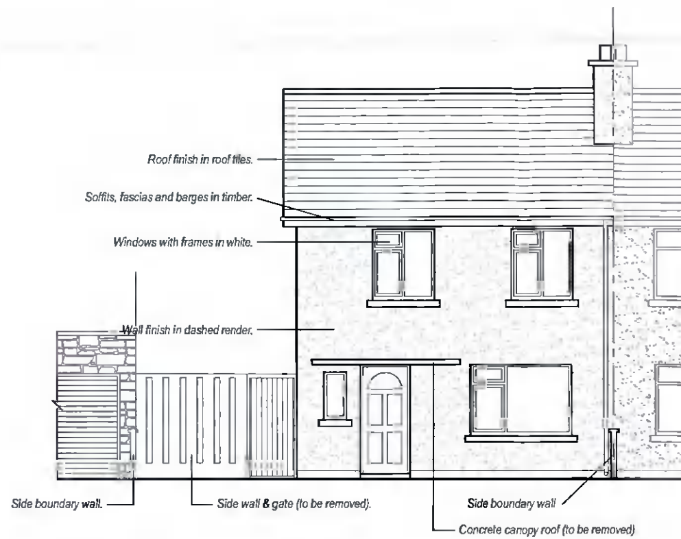
EXISTING SOUTHEAST ELEVATION - FRONT SCALE - 1 : 100
