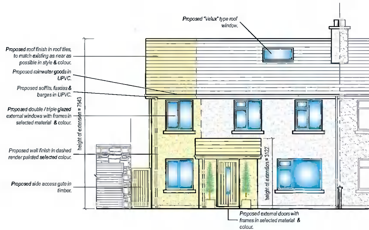
PROPOSED SOUTHEAST ELEVATION - FRONT SCALE - 1 : 100
