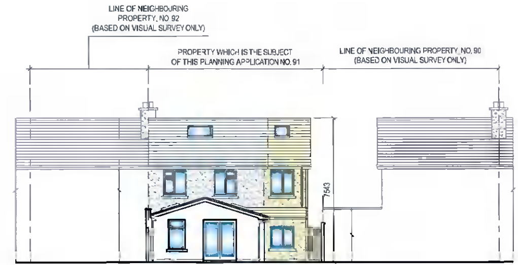
PROPOSED NORTHWEST ELEVATION - REAR CONTIGUOUS ELEVATIONS SCALE - 1 : 200
