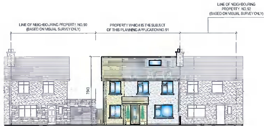
PROPOSED SOUTHEAST ELEVATION - FRONT CONTIGUOUS ELEVATIONS SCALE - 1 : 200
