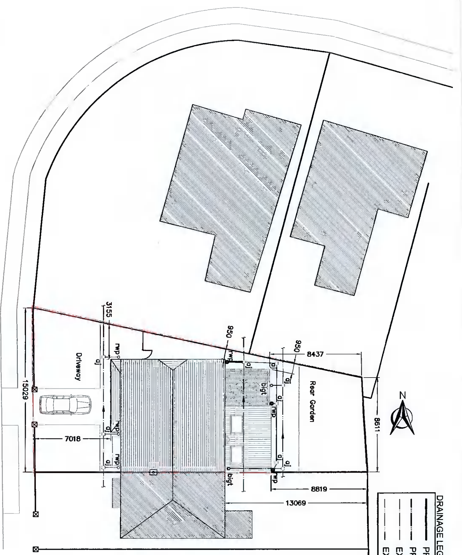
Proposed Block Plan & Drainage Layout SCALE 1:200
