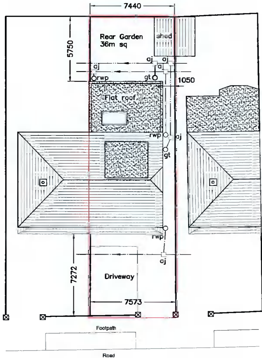
Proposed Block Plan & Drainage Layout SCALE 1:200
