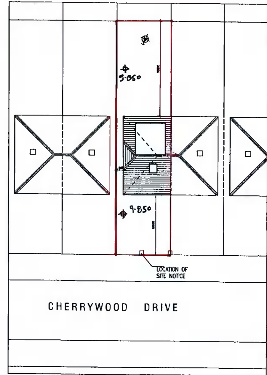
PROPOSED ROOF/SITE PLAN 1-250
