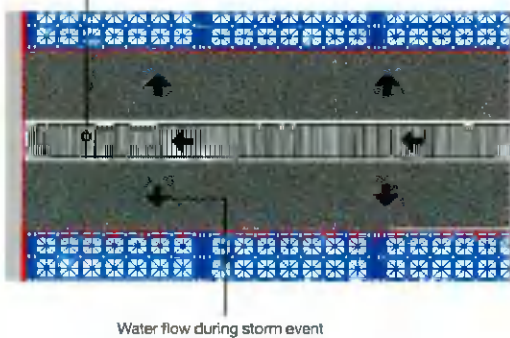
Wavin TwinWall half-perforated pipe
