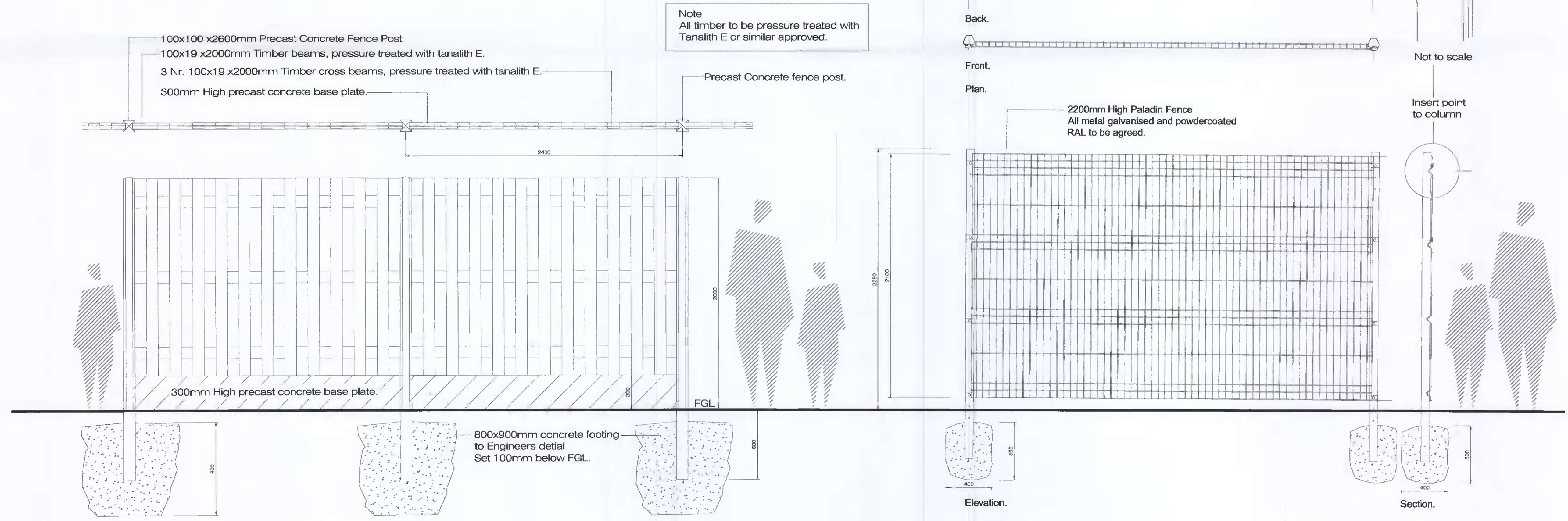
Detail D 02 Dwg BD-01-PP 2.0mtr High concrete post with hit + miss timber panel fence and precast concrete kicker board to rear gardens Scale @ 1:25
