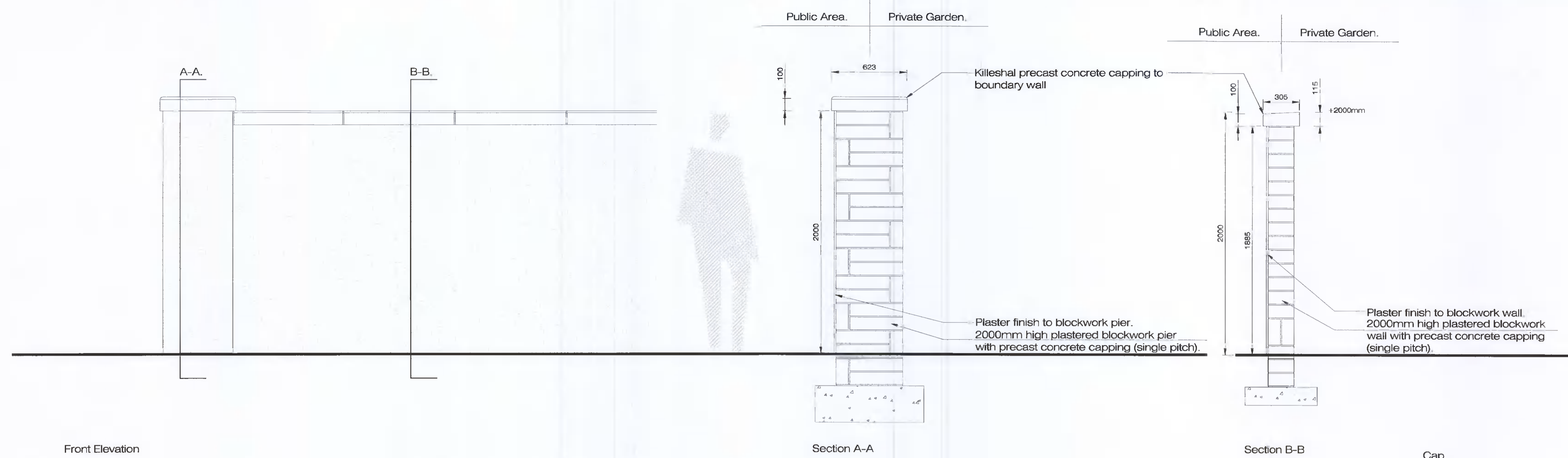
Detail D01 Dwg BD-01-PP 2.0mtr Rendered Blockwall boundary between rear garden and public open space and public pathways Scale @ 1:20
