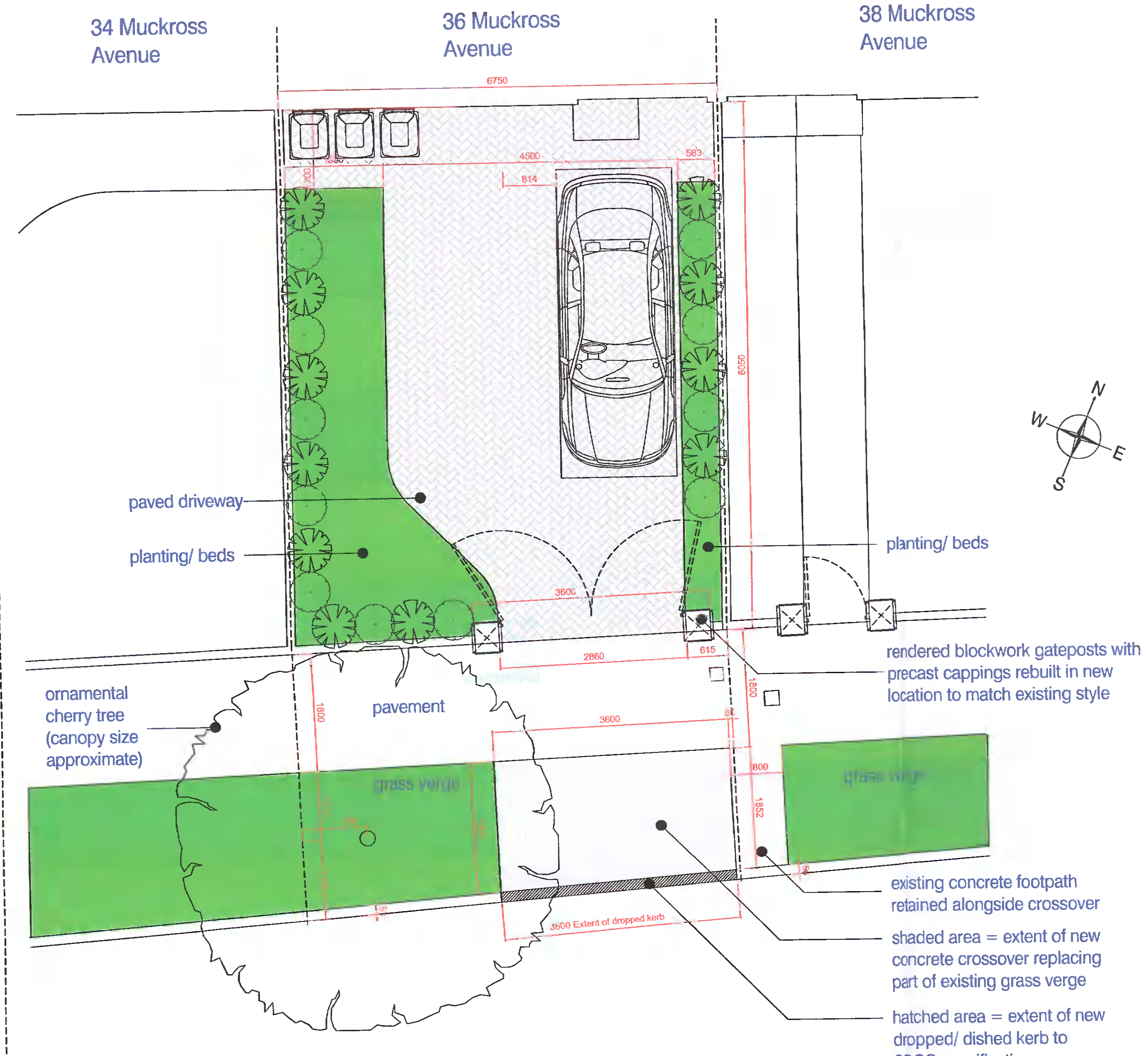
PROPOSED PLAN
