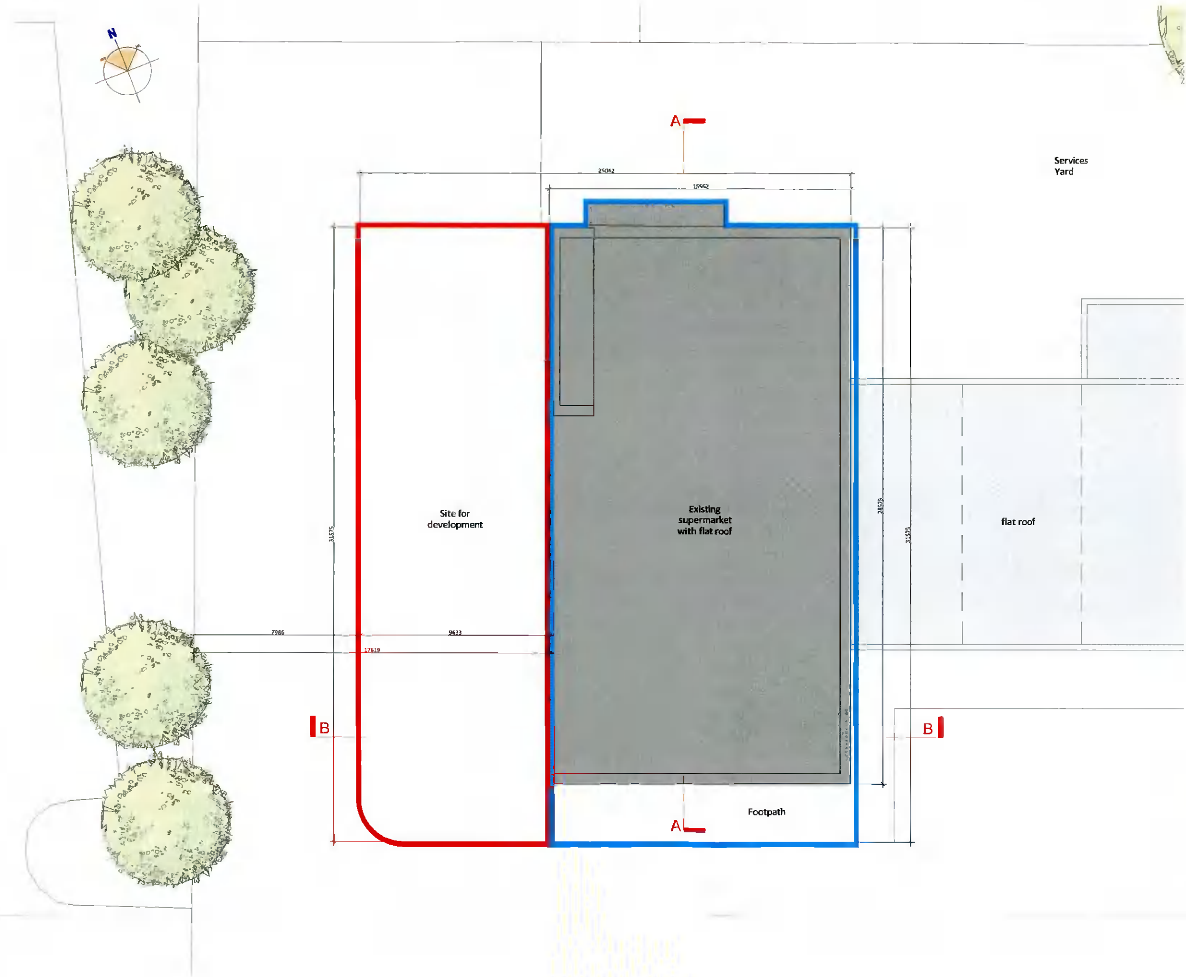
Existing Roof Plan 1:200
