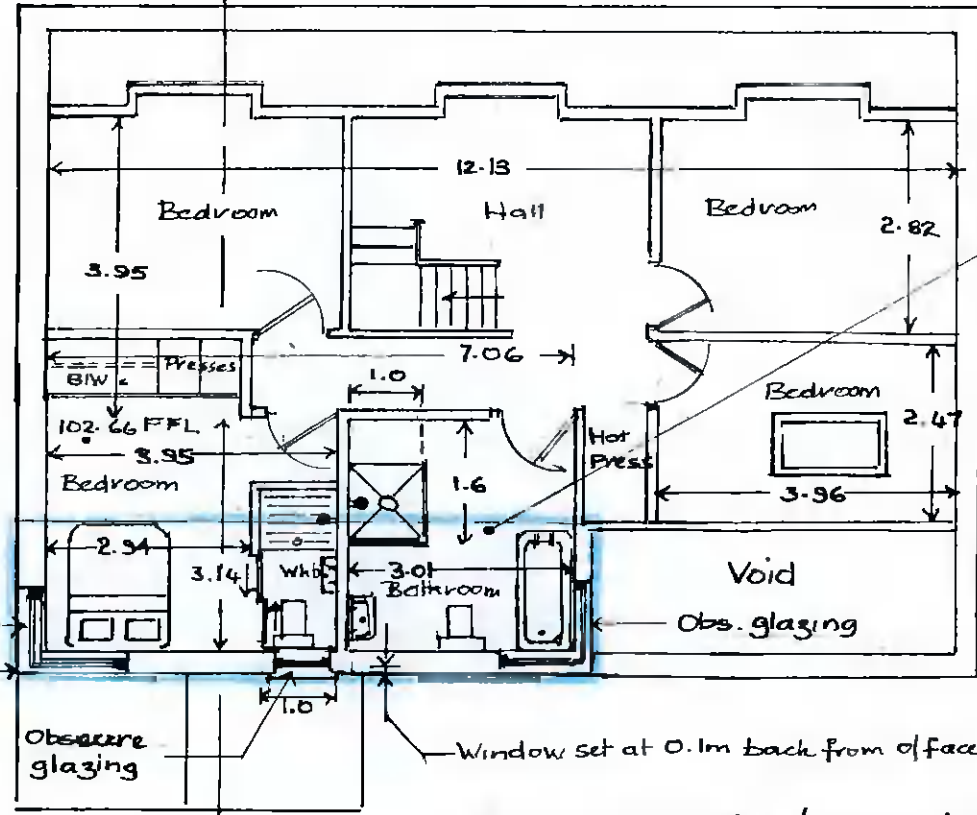
Proposed First Floor/Dormer 1=100 Extension outlined blue
