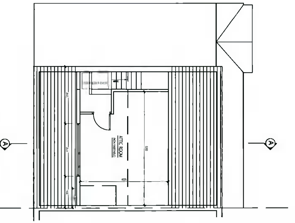
PROPOSED ATTIC FLOOR PLAN
