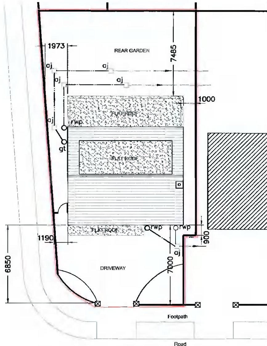
Proposed Block Plan & Drainage Layout SCALE 1:200
