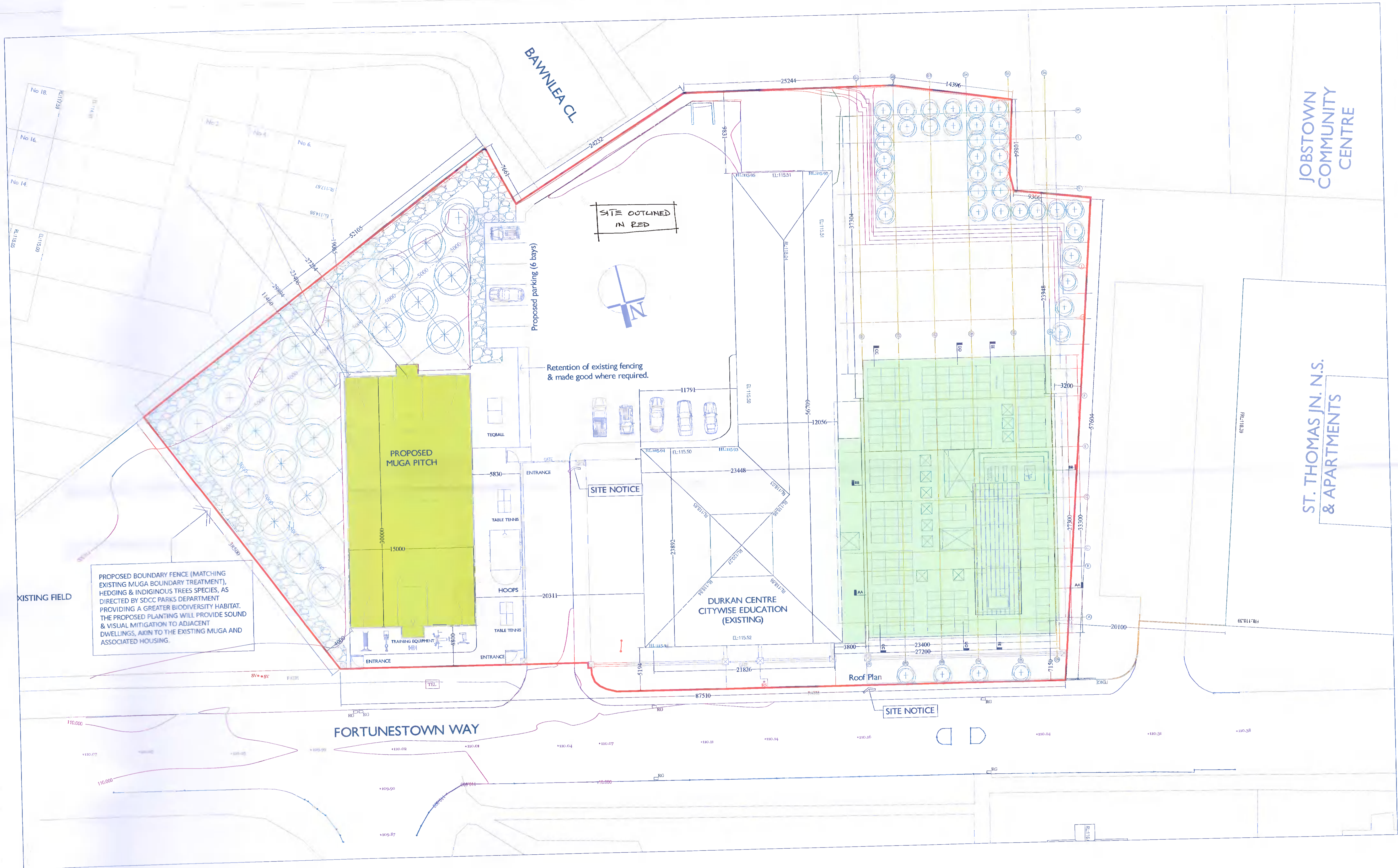
PROPOSED SITE LAYOUT PLAN 1-200 (Site outlined in red)
