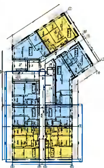
1 Block F2 Proposed Ground Floor Plan PART V 1:200
