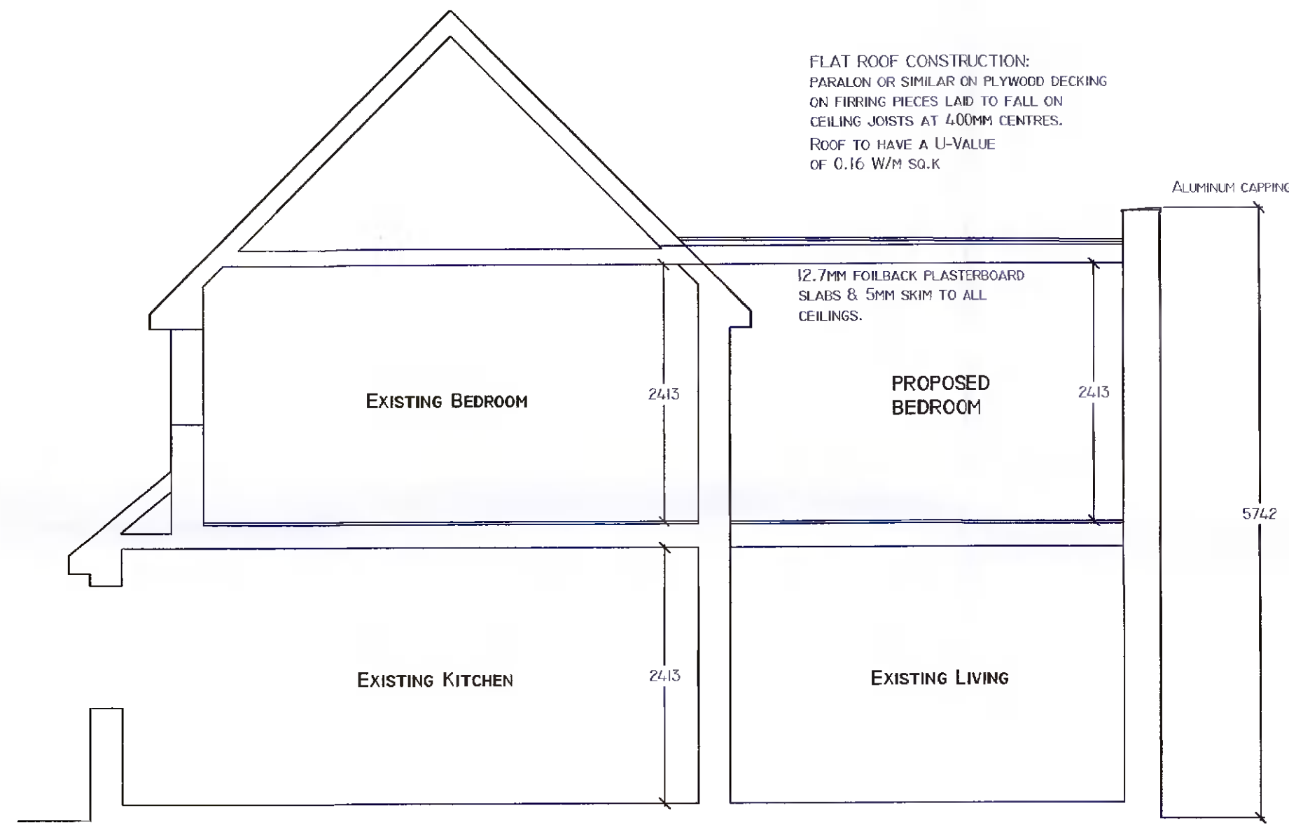
PROPOSED TYPICAL SECTION SCALE 1:50
