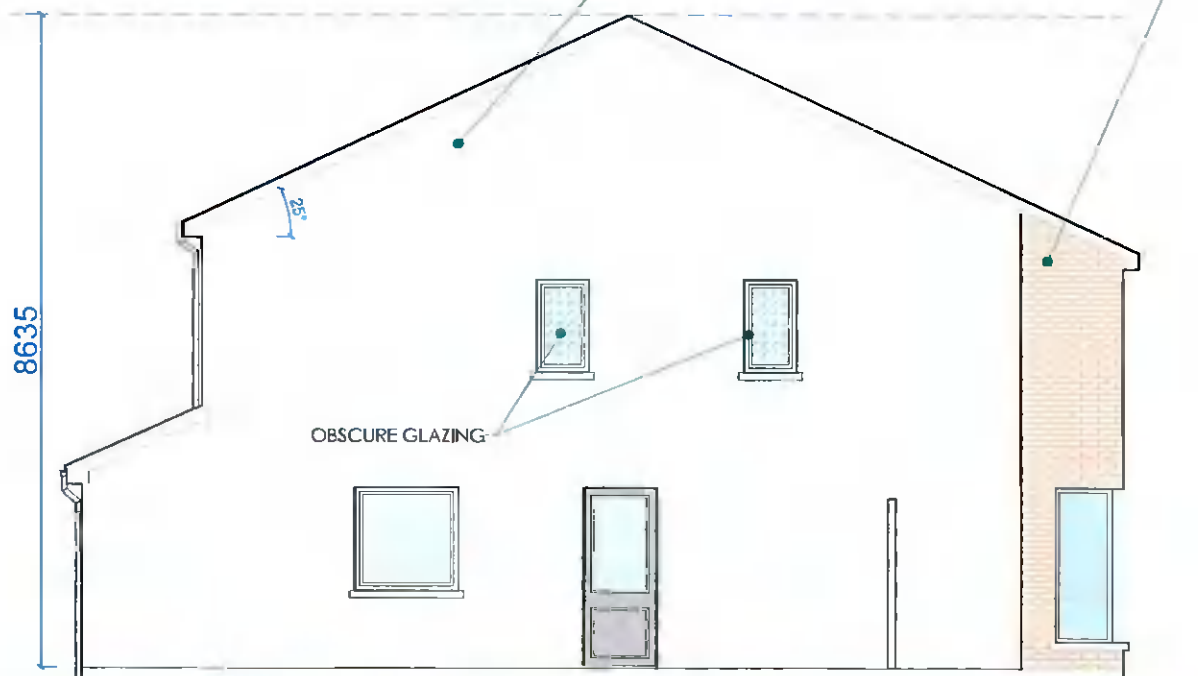
SIDE ELEVATION - house type A
