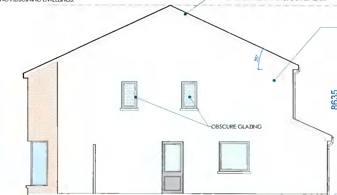
SIDE ELEVATION - house type A
