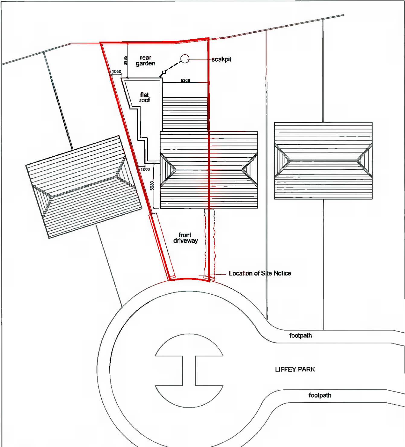
PROPOSED SITE LAYOUT PLAN Scale:1:250
