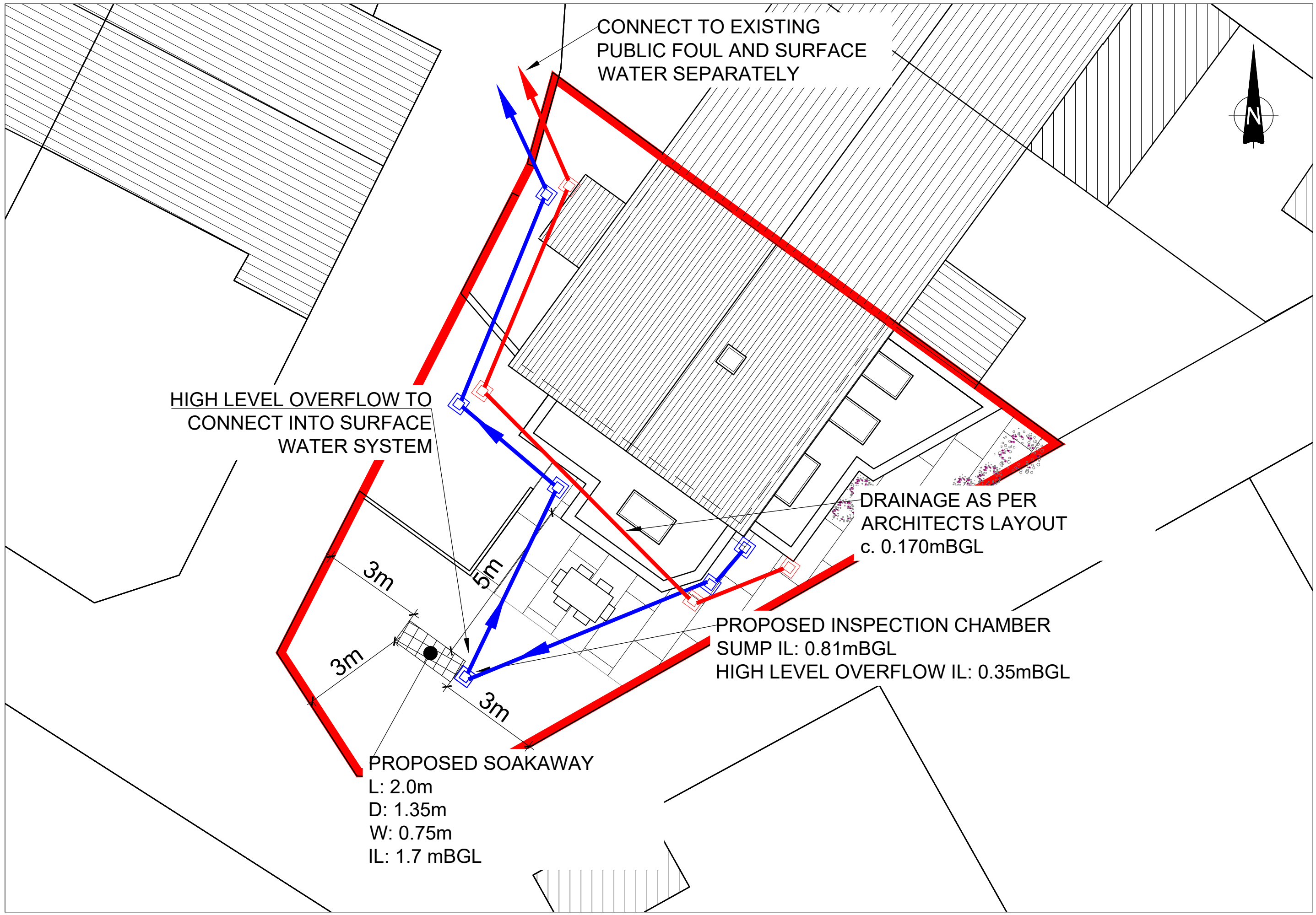
PLAN VIEW - PROPOSED SOAKAWAY LOCATION SCALE 1:100
