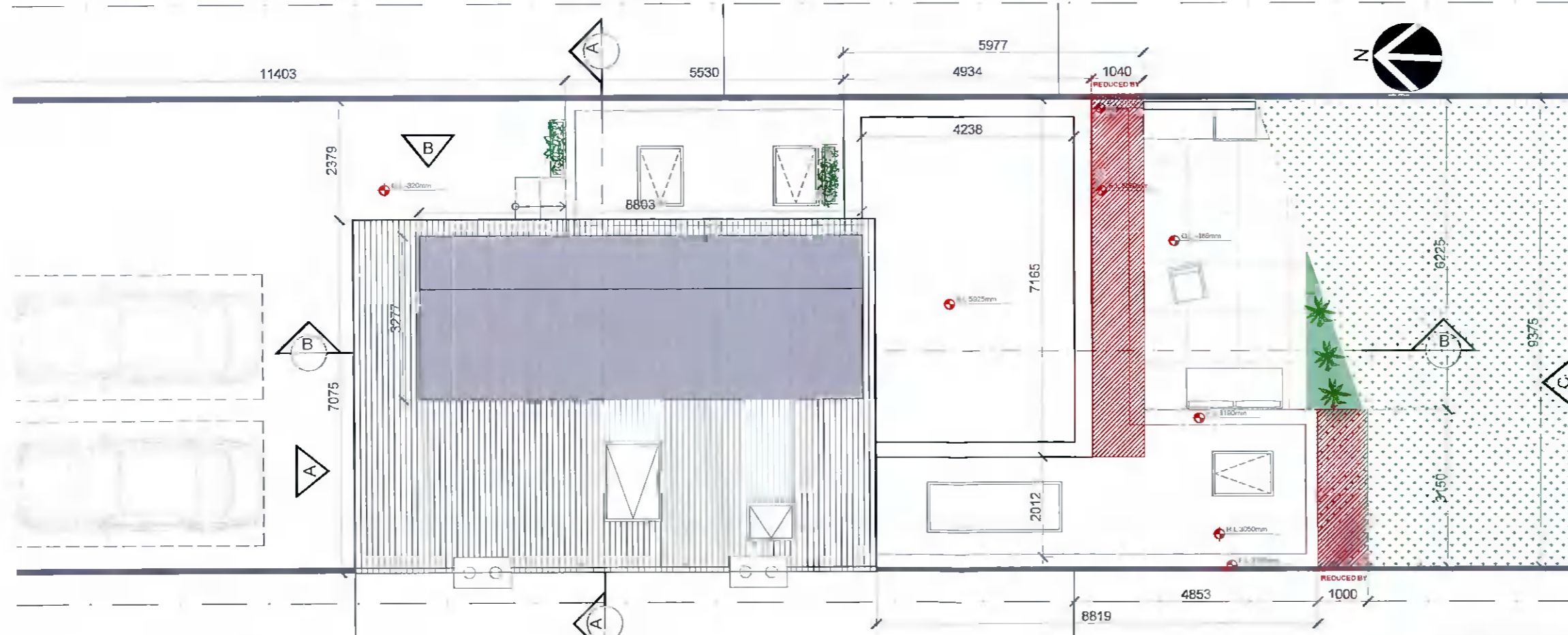
02 PROPOSED ROOF PLAN SCALE: 1:100
