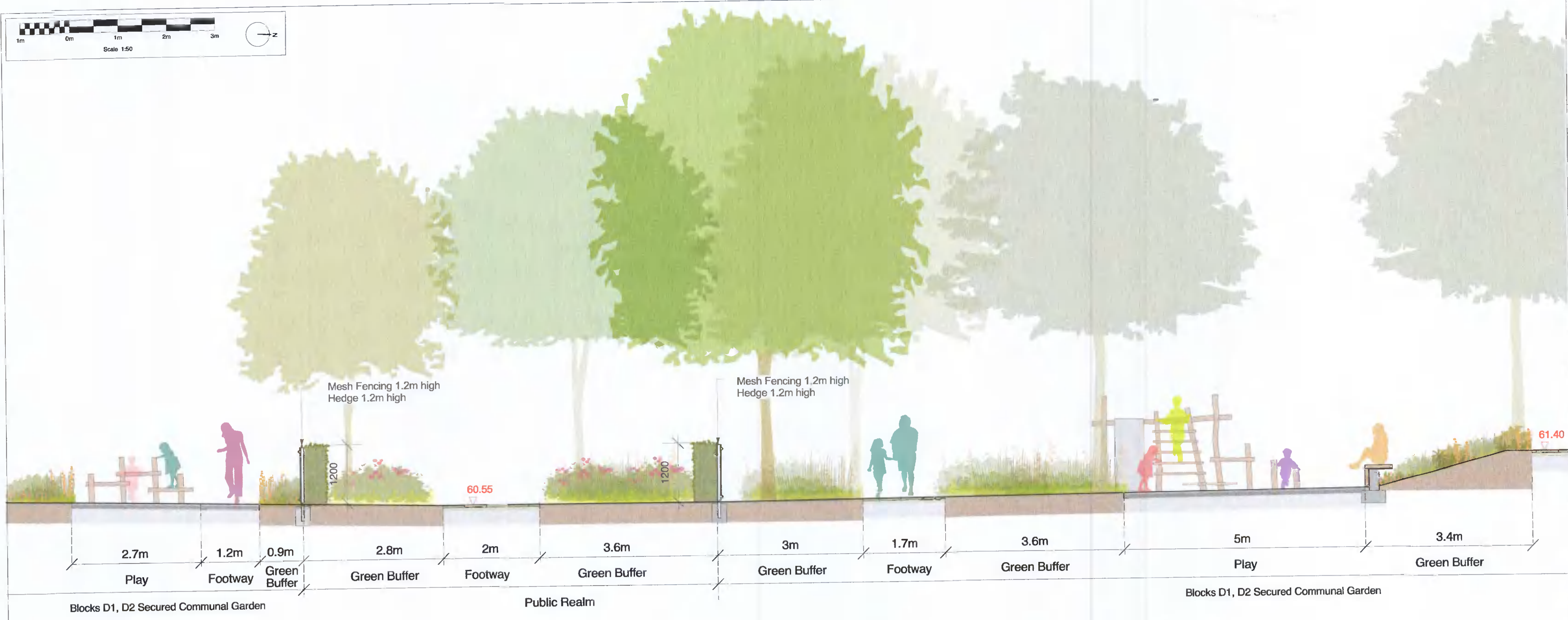
Section F Of Public Realm And Block D Communal Garden Scale 1:50 at A1
