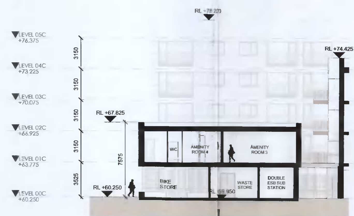
P Pavillion Section North/South 1: 200
