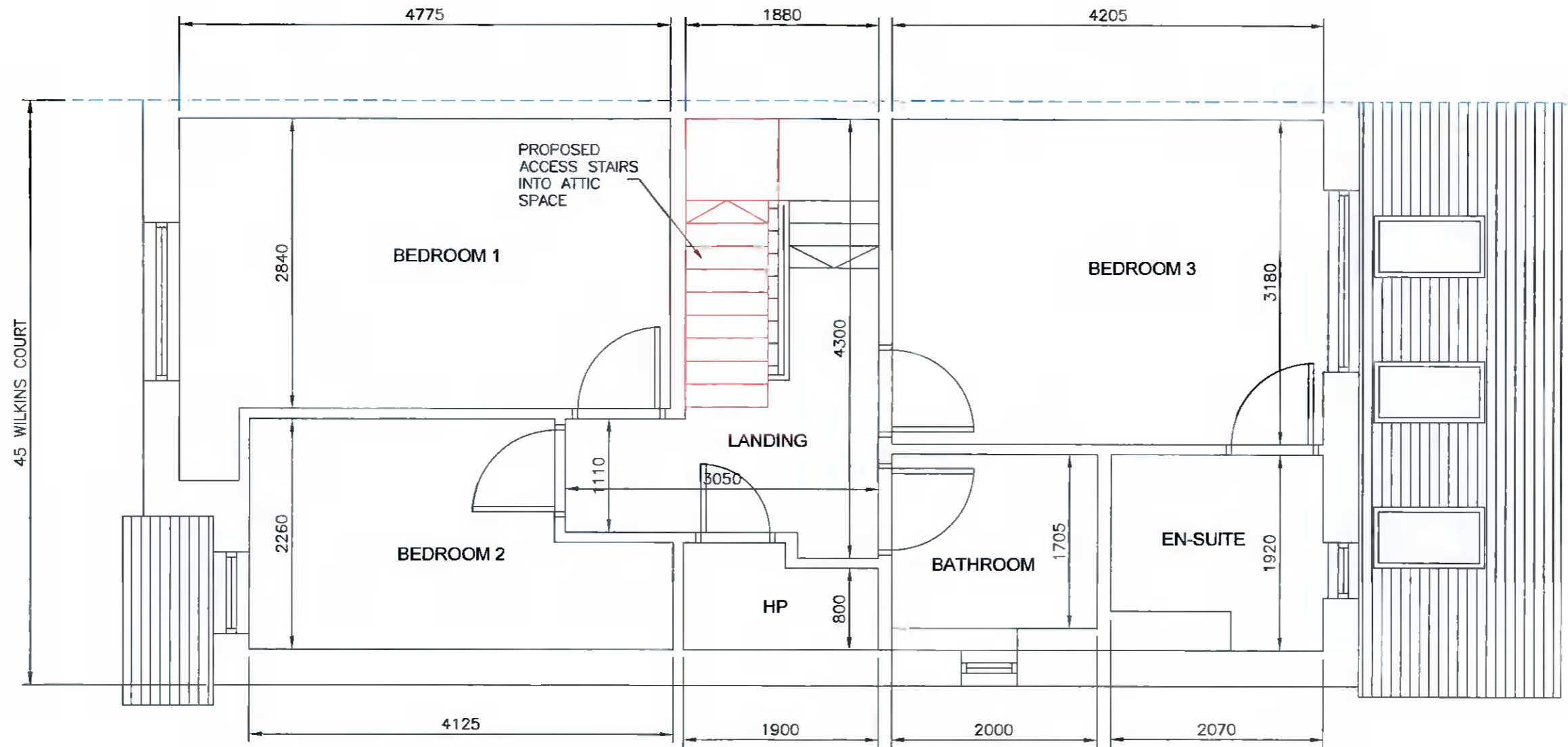
PROPOSED FIRST FLOOR PLAN VIEW
