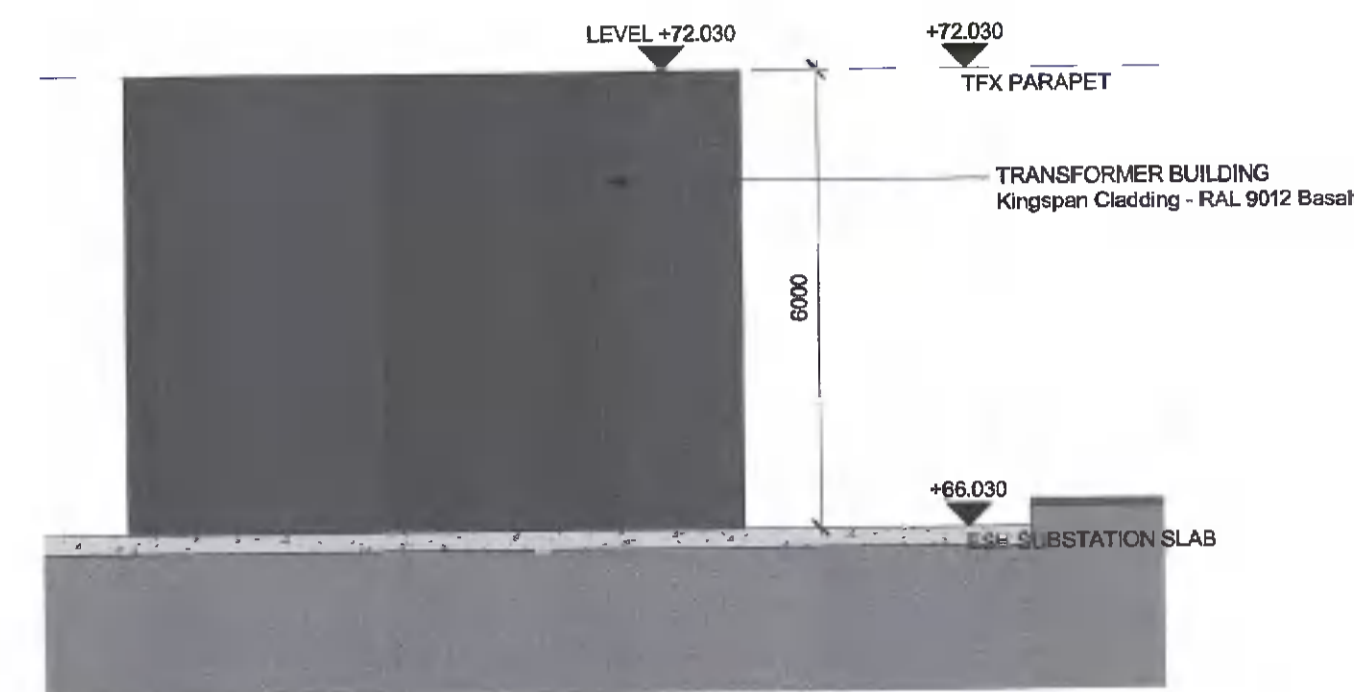
2 PERMITTED GA - TRANSFORMER BUILDING - EAST ELEVATION SCALE: 1:100
