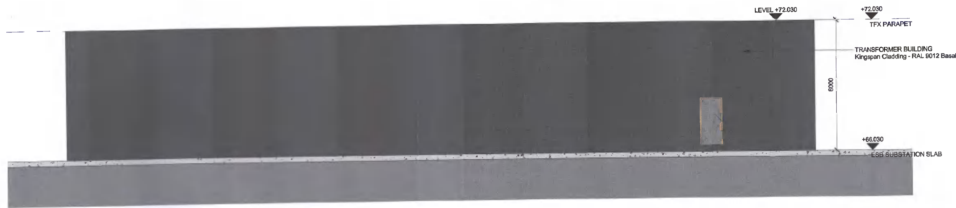
1 PERMITTED GA - TRANSFORMER BUILDING - NORTH ELEVATION SCALE: 1:100
