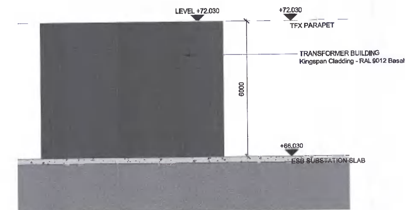
4 PERMITTED GA - TRANSFORMER BUILDING - WEST ELEVATION SCALE: 1:100
