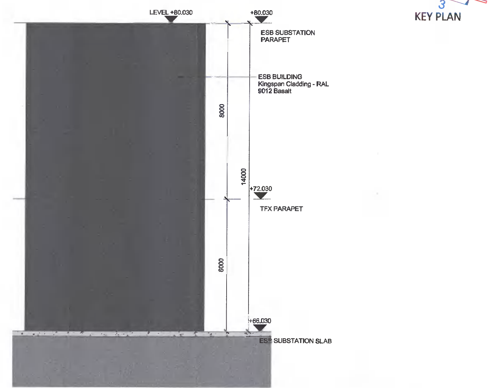
2 PERMITTED GA - ESB BUILDING - EAST ELEVATION SCALE: 1:100
