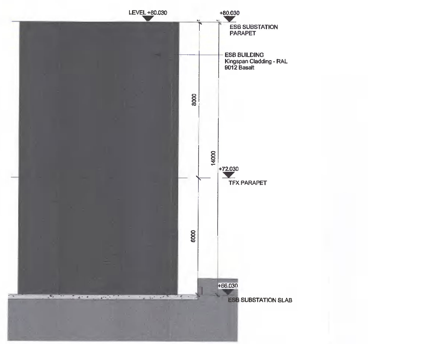
4 PERMITTED GA - ESB BUILDING - WEST ELEVATION SCALE: 1:100
