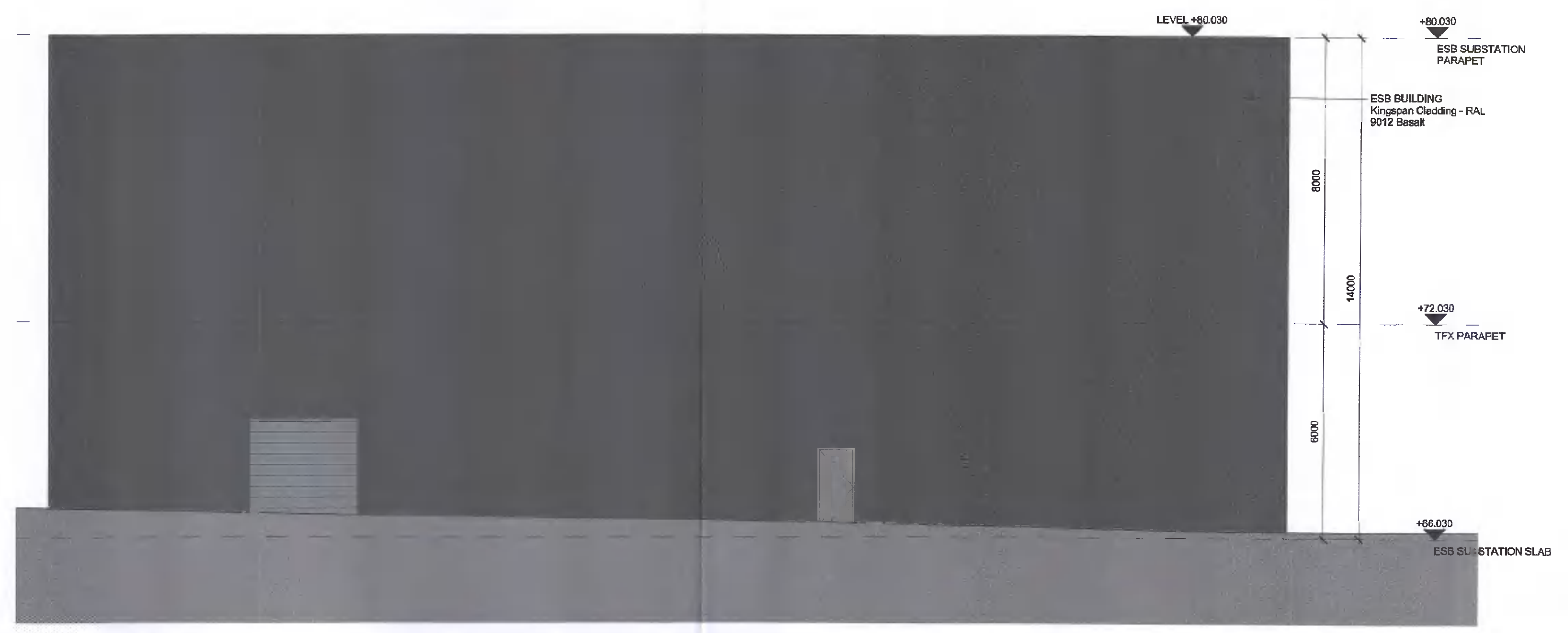
3 PERMITTED GA - ESB BUILDING - SOUTH ELEVATION SCALE: 1:100
