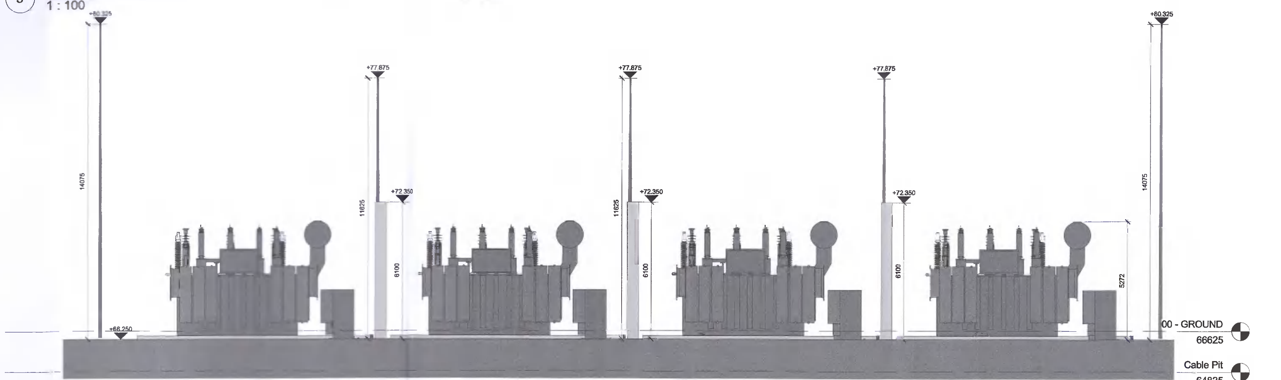
4 GA - TRANSFORMER YARD - SOUTH ELEVATION 1 : 100
