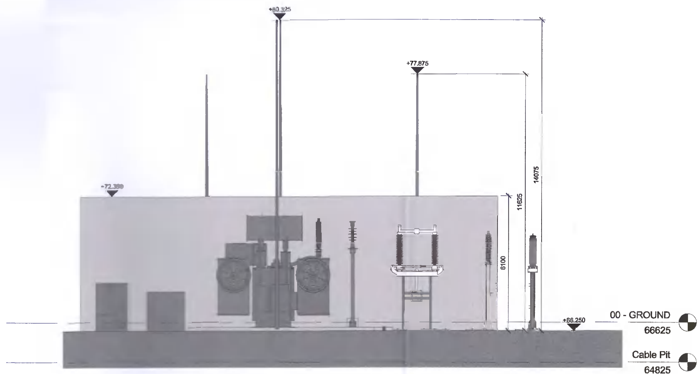
1 GA - TRANSFORMER YARD - EAST ELEVATION 1 : 100
