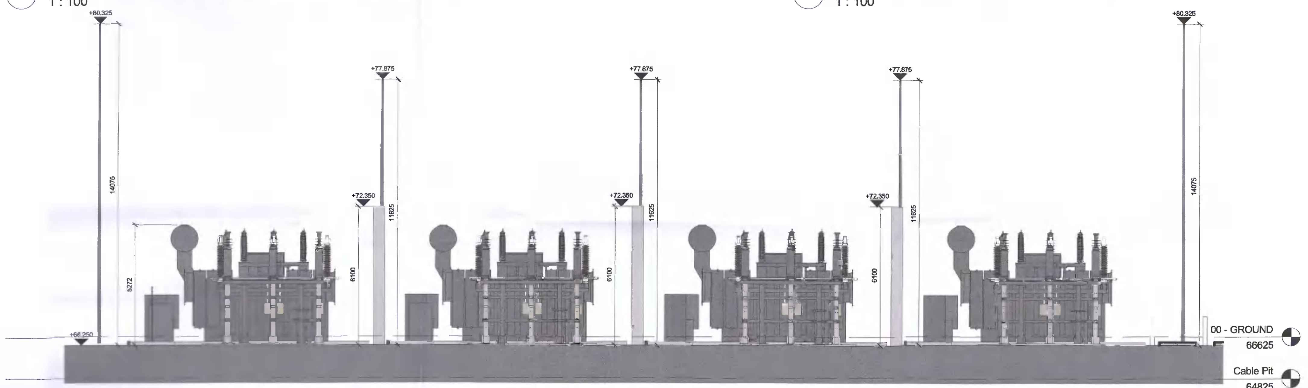
3 GA - TRANSFORMER YARD - NORTH ELEVATION 1 : 100
