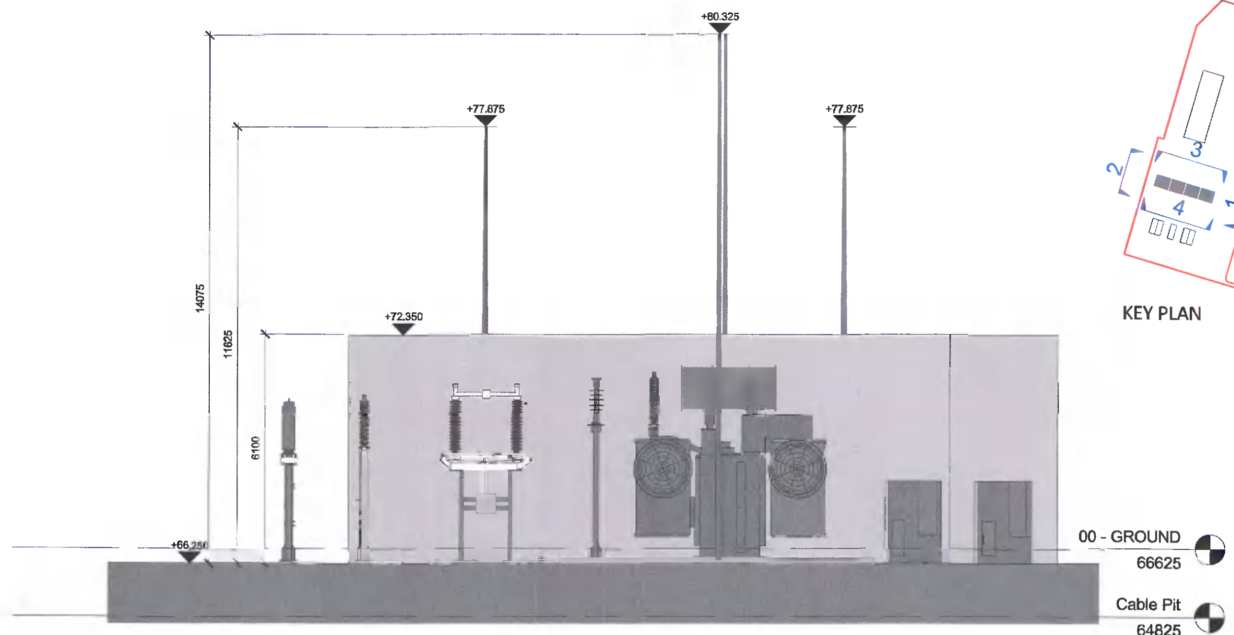
2 GA - TRANSFORMER YARD - WEST ELEVATION 1 : 100
