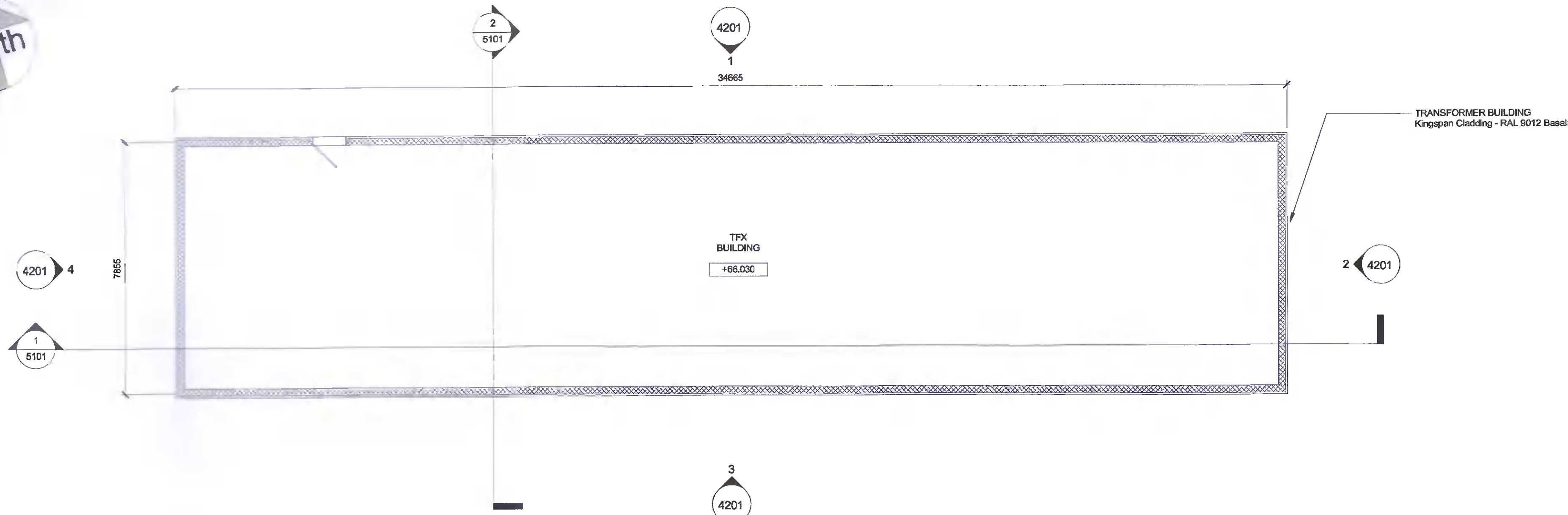
1 PERMITTED GA - TRANSFORMER BUILDING GROUND FLOOR PLAN SCALE: 1 : 100
