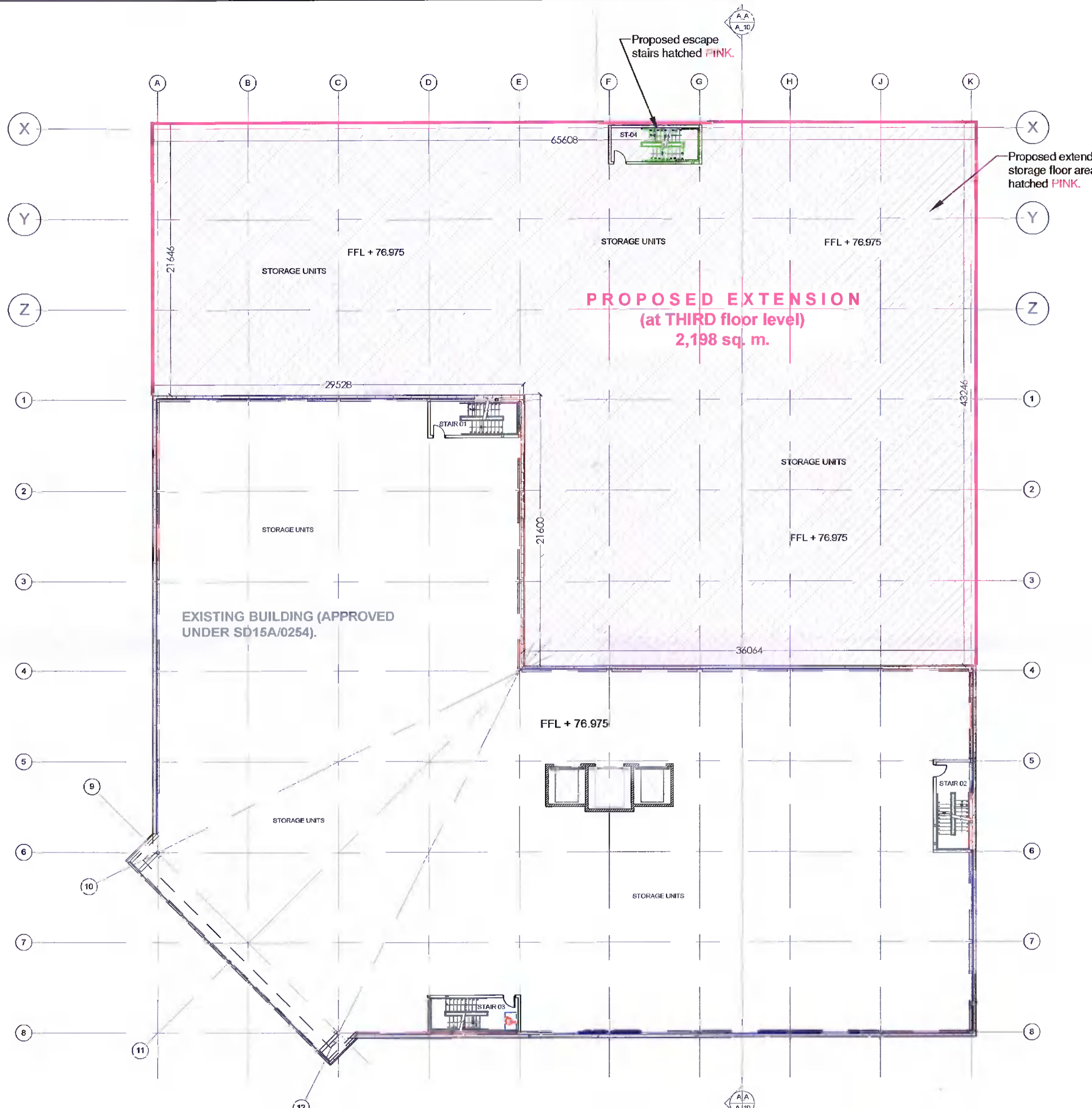
Third Floor Plan (Scale 1:250).
