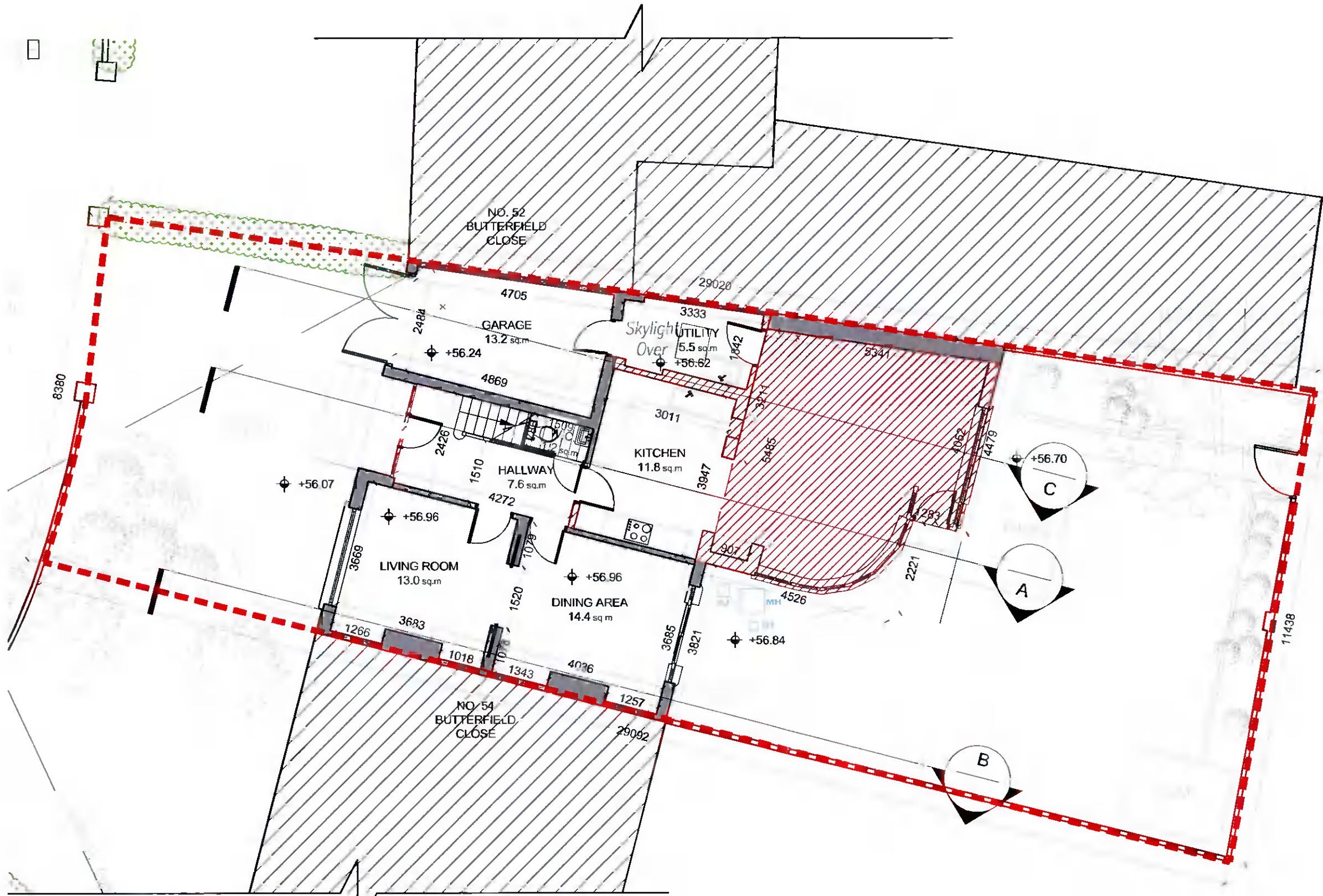
EXISTING / DEMOLITION SITE LAYOUT & GROUND FLOOR PLAN 1:100
