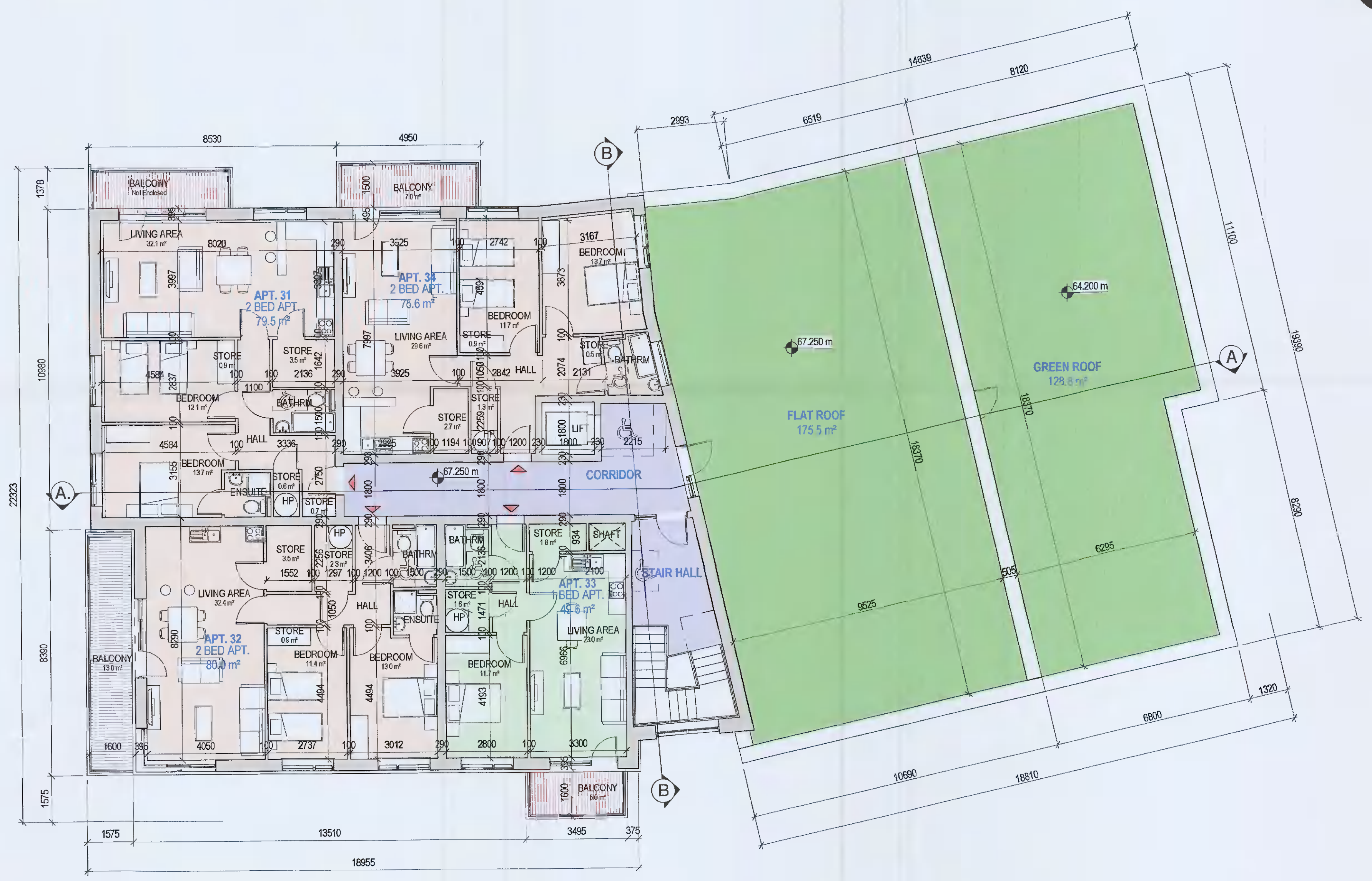
BLOCK 2 FOURTH FLOOR PLAN 1 : 100
